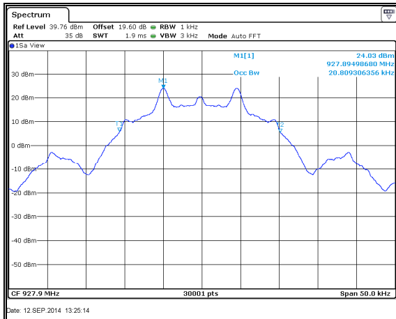
Figure 7.4.4.2-36: 99% BW High Channel – 9.6kbps
