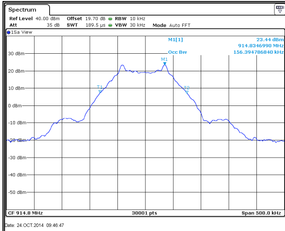
Figure 7.4.4.2-34: 99% BW Mid Channel – 150.0kbps
