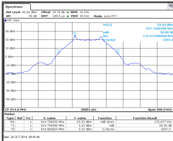
Figure 7.4.4.2-13: 20dB BW Mid Channel – 150.0kbps
