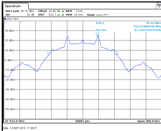
Figure 7.4.4.2-31: 99% BW Mid Channel – 38.4kbps
