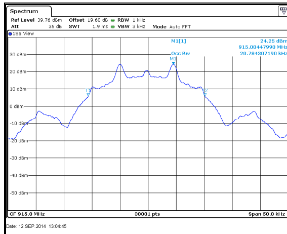
Figure 7.4.4.2-29: 99% BW Mid Channel – 9.6kbps
