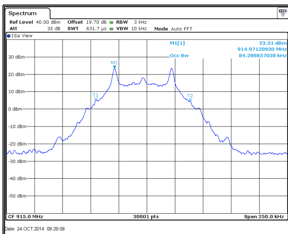
Figure 7.4.4.2-32: 99% BW Mid Channel – 50.0kbps
