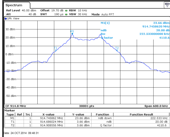
Figure 7.4.4.2-14: 20dB BW Mid Channel – 200.0kbps
