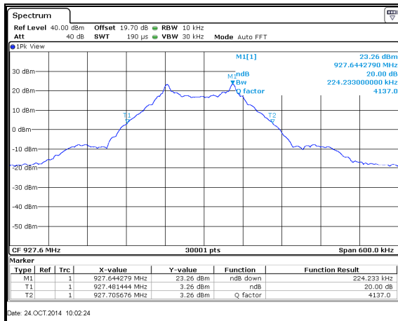
Figure 7.4.4.2-21: 20dB BW High Channel – 200.0kbps
