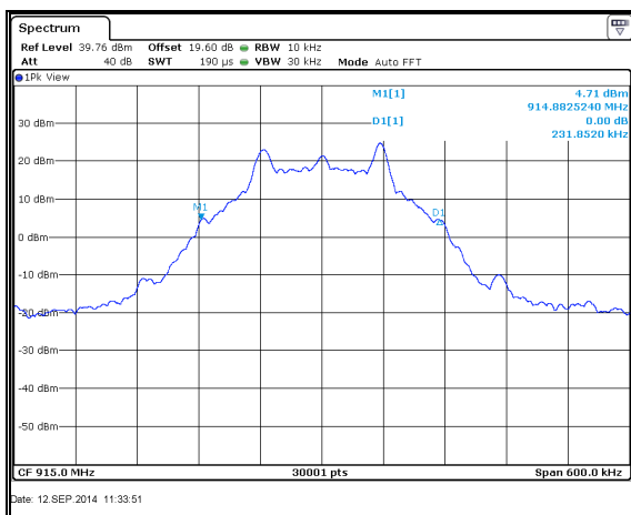
Figure 7.4.4.2-12: 20dB BW Mid Channel – 115.2kbps
