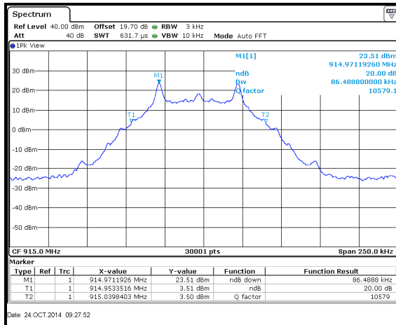
Figure 7.4.4.2-11: 20dB BW Mid Channel – 50.0kbps
