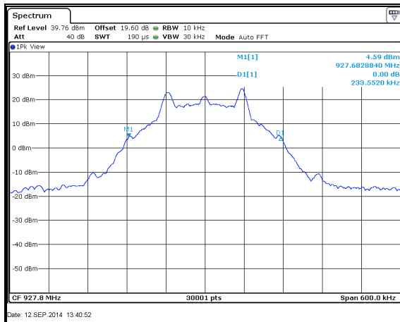
Figure 7.4.4.2-19: 20dB BW High Channel – 115.2kbps
