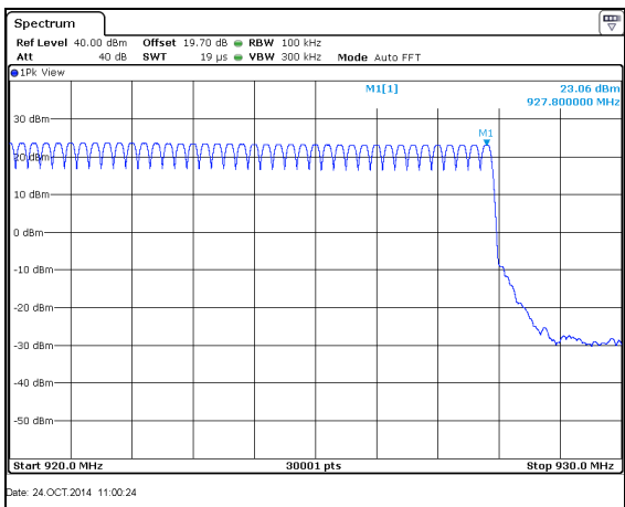
Figure 7.4.2.2-10: Mode 3 (129 Channels)
