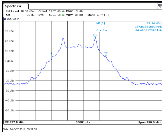
Figure 7.4.4.2-39: 99% BW High Channel – 50.0kbps
