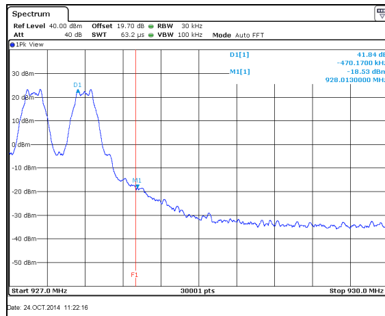
Figure 7.5.1.2-16: Upper Band-edge – Mode 4
