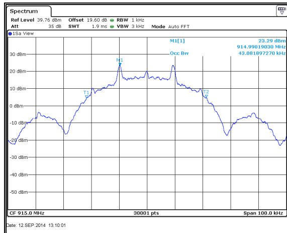
Figure 7.4.4.2-30: 99% BW Mid Channel – 19.2kbps
