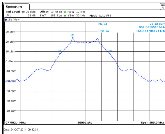
Figure 7.4.4.2-27: 99% BW Low Channel – 150.0kbps
