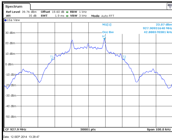
Figure 7.4.4.2-37: 99% BW High Channel – 19.2kbps
