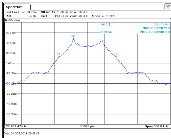
Figure 7.4.4.2-28: 99% BW Low Channel – 200.0kbps
