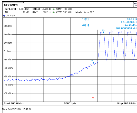
Figure 7.5.1.2-11: Lower Band-edge – Mode 3
