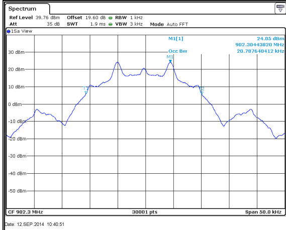
Figure 7.4.4.2-22: 99% BW Low Channel – 9.6kbps
