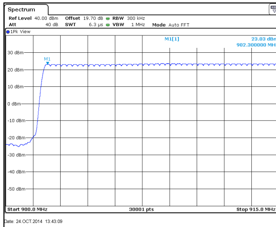
Figure 7.4.2.2-1: Mode 1 (86 Channels)
