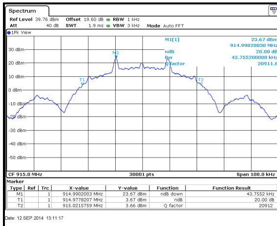
Figure 7.4.4.2-9: 20dB BW Mid Channel – 19.2kbps
