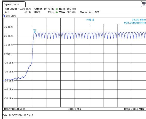
Figure 7.4.2.2-8: Mode 3 (129 Channels)
