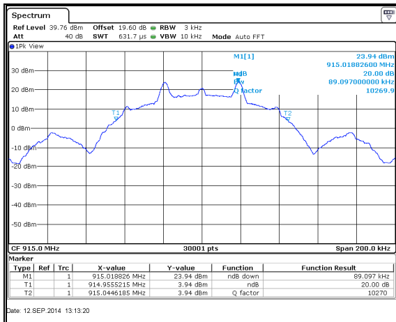
Figure 7.4.4.2-10: 20dB BW Mid Channel – 38.4kbps
