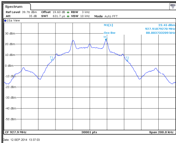
Figure 7.4.4.2-38: 99% BW High Channel – 38.4kbps
