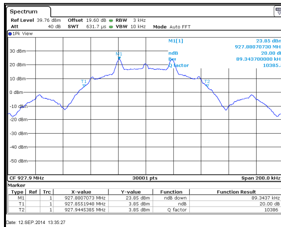
Figure 7.4.4.2-17: 20dB BW High Channel – 38.4kbps
