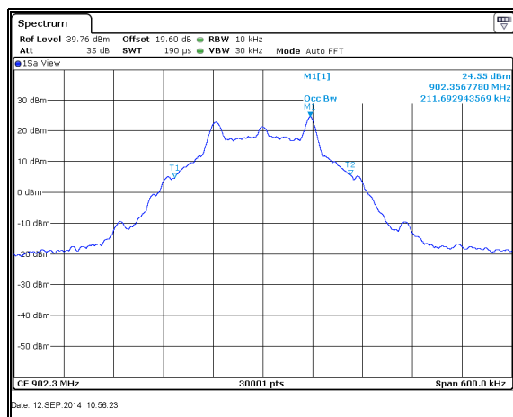
Figure 7.4.4.2-26: 99% BW Low Channel – 115.2kbps
