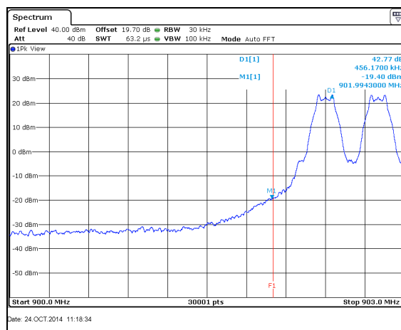
Figure 7.5.1.2-12: Lower Band-edge – Mode 4
