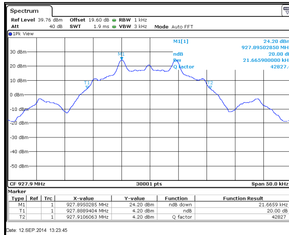
Figure 7.4.4.2-15: 20dB BW High Channel – 9.6kbps
