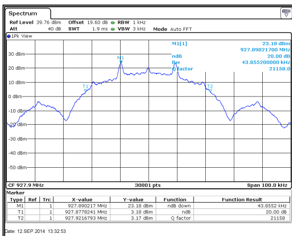
Figure 7.4.4.2-16: 20dB BW High Channel – 19.2kbps
