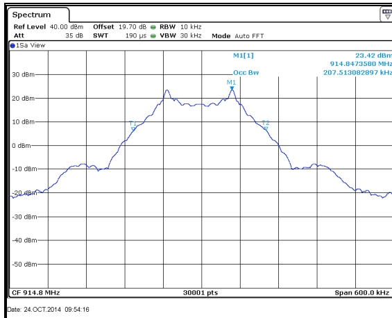
Figure 7.4.4.2-35: 99% BW Mid Channel – 200.0kbps
