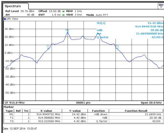
Figure 7.4.4.2-8: 20dB BW Mid Channel – 9.6kbps
