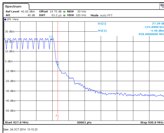
Figure 7.5.1.2-14: Upper Band-edge – Mode 2
