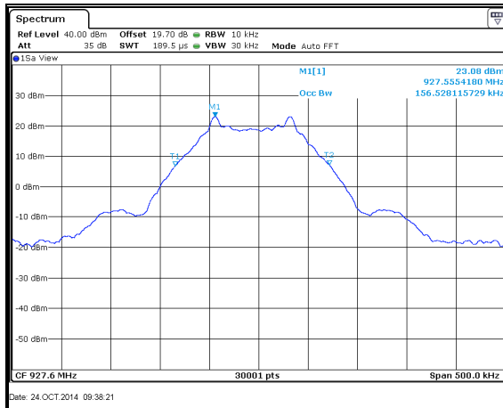
Figure 7.4.4.2-41: 99% BW High Channel – 150.0kbps
