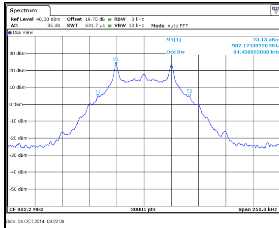
Figure 7.4.4.2-25: 99% BW Low Channel – 50.0kbps
