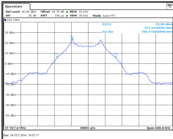
Figure 7.4.4.2-42: 99% BW High Channel – 200.0kbps
