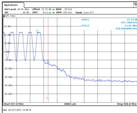
Figure 7.5.1.2-15: Upper Band-edge – Mode 3
