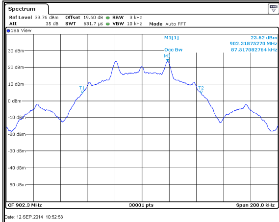
Figure 7.4.4.2-24: 99% BW Low Channel – 38.4kbps
