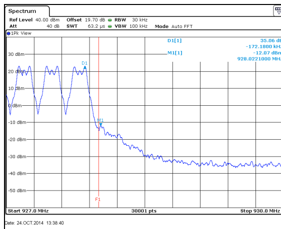
Figure 7.5.1.2-13: Upper Band-edge – Mode 1
