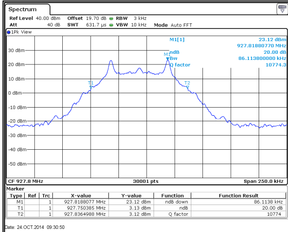
Figure 7.4.4.2-18: 20dB BW High Channel – 50.0kbps
