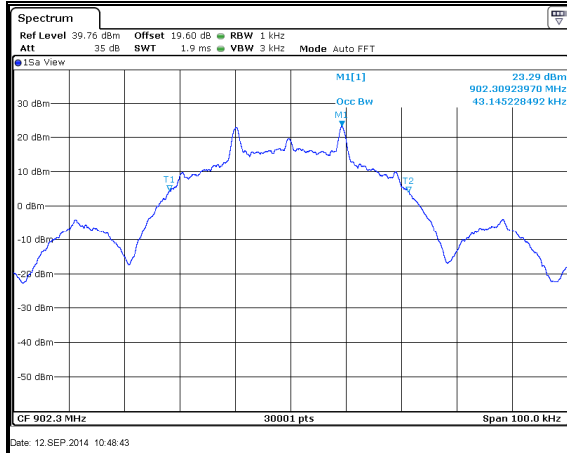
Figure 7.4.4.2-23: 99% BW Low Channel – 19.2kbps
