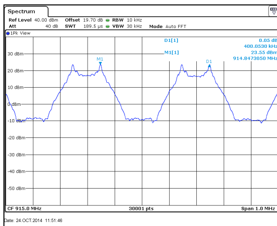
Figure 7.4.1.2-4: Mode 4
