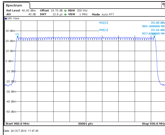
Figure 7.4.2.2-11: Mode 4 (64 Channels)
