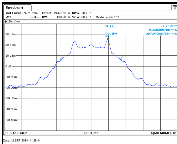
Figure 7.4.4.2-33: 99% BW Mid Channel – 115.2kbps
