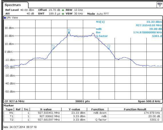
Figure 7.4.4.2-20: 20dB BW High Channel – 150.0kbps
