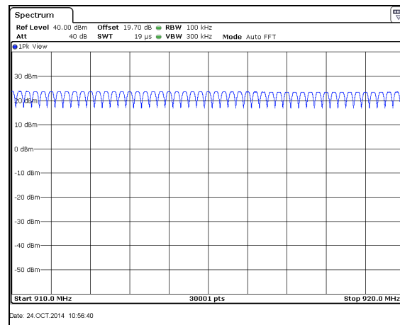
Figure 7.4.2.2-9: Mode 3 (129 Channels)
