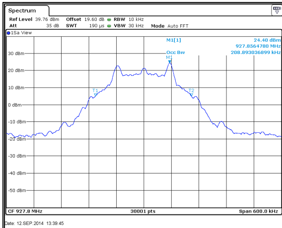
Figure 7.4.4.2-40: 99% BW High Channel – 115.2kbps
