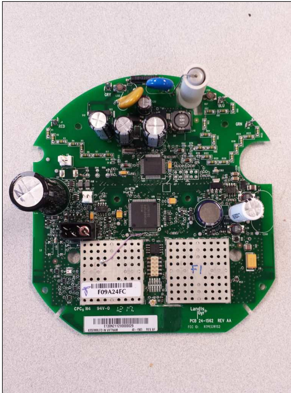
Figure 2: Internal Photo – PCB with Shields
