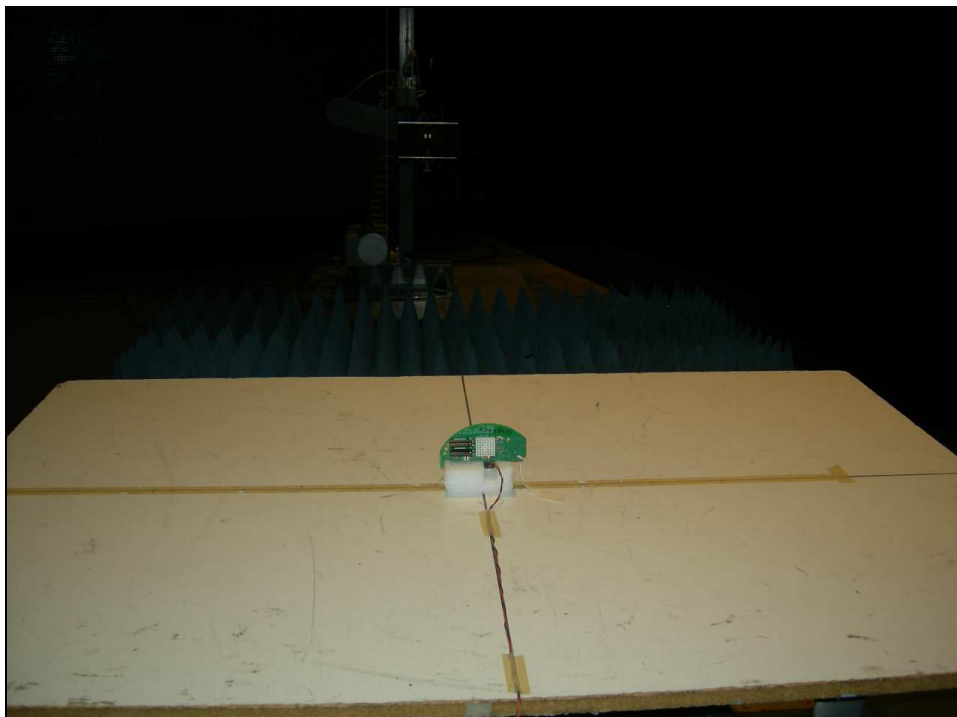
Figure 2: Radiated Emissions
