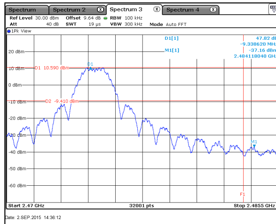
Figure 7.5.1.2-5: Upper Band-edge - 2475 MHz
