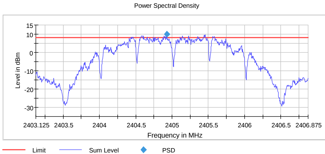
Figure 7.6.2-1: Sample PSD Plot (10kHz RBW)
