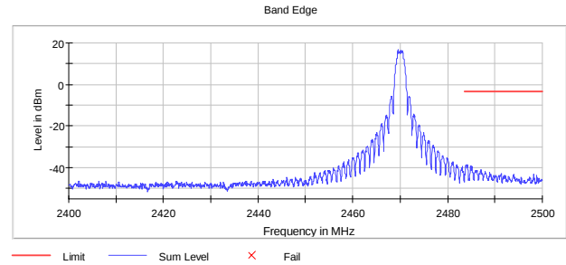
Figure 7.5.1.2-5: Upper Band-edge – Channel 24
