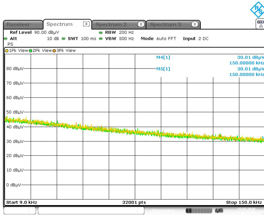
Figure A-1: 9kHz-150kHz
