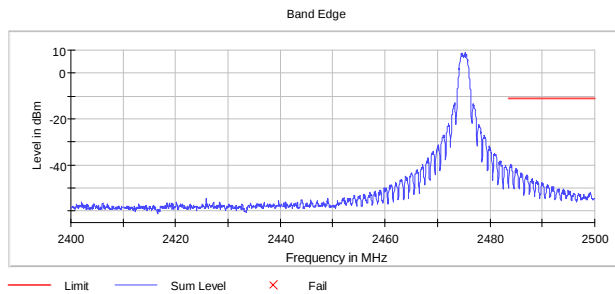
Figure 7.5.1.2-6: Upper Band-edge – Channel 25
