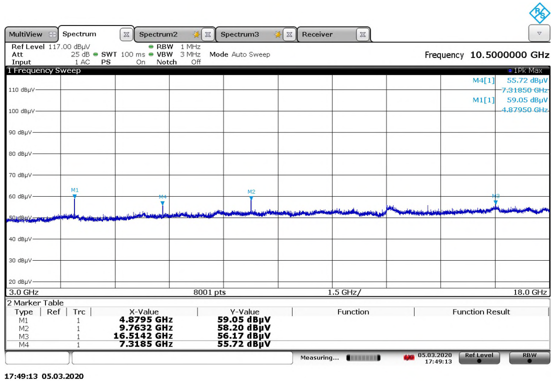
Figure A-5: 3GHz-18GHz
