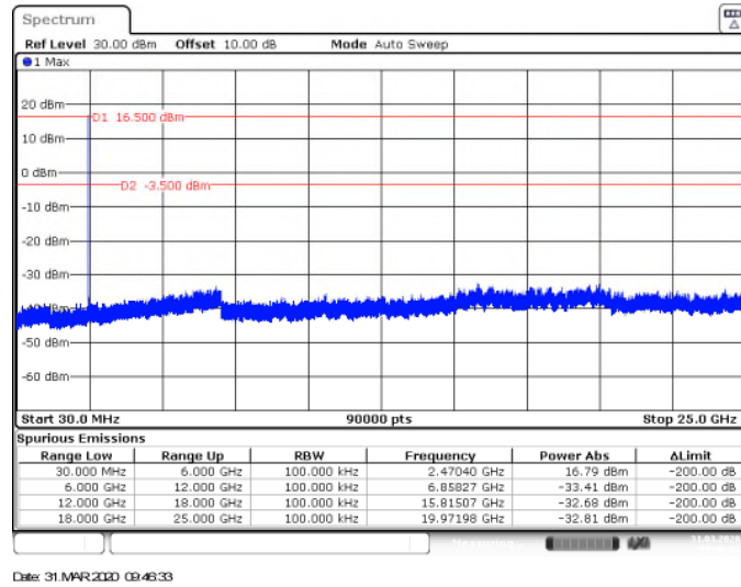
Figure 7.5.1.2-3: HCH (2470MHz) – 30MHz–25GHz
