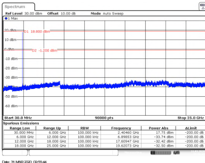
Figure 7.5.1.2-1: LCH (2405MHz) – 30MHz–25GHz
