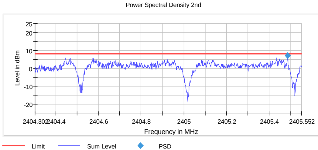
Figure 7.6.2-2: Sample PSD Plot (3kHz RBW)
