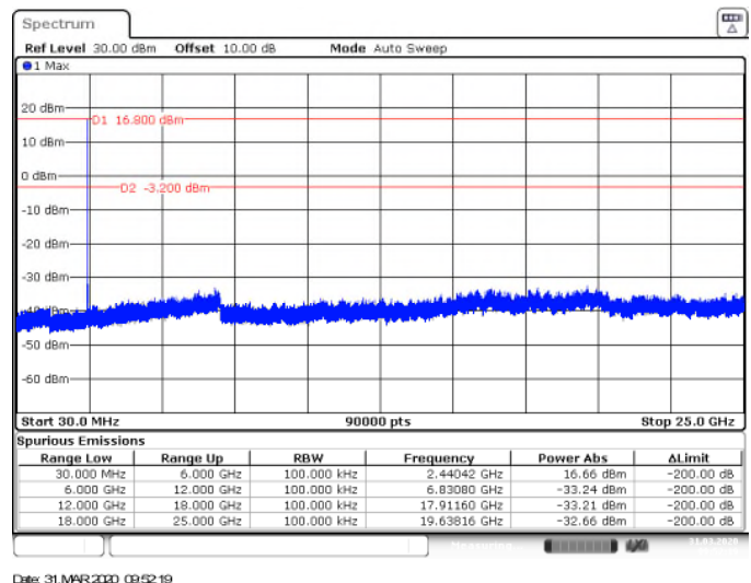
Figure 7.5.1.2-2: MCH (2440MHz) – 30MHz–25GHz
