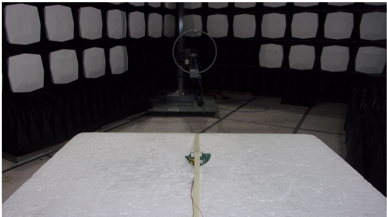
Figure 2: Equipment Under Test – Radiated Emissions <30MHz
