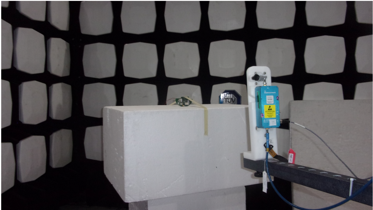
Figure 7: Equipment Under Test – Radiated Emissions >18GHz
