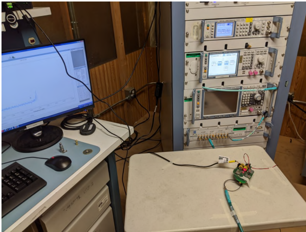
Figure 7: Equipment Under Test – Antenna Port Conducted
