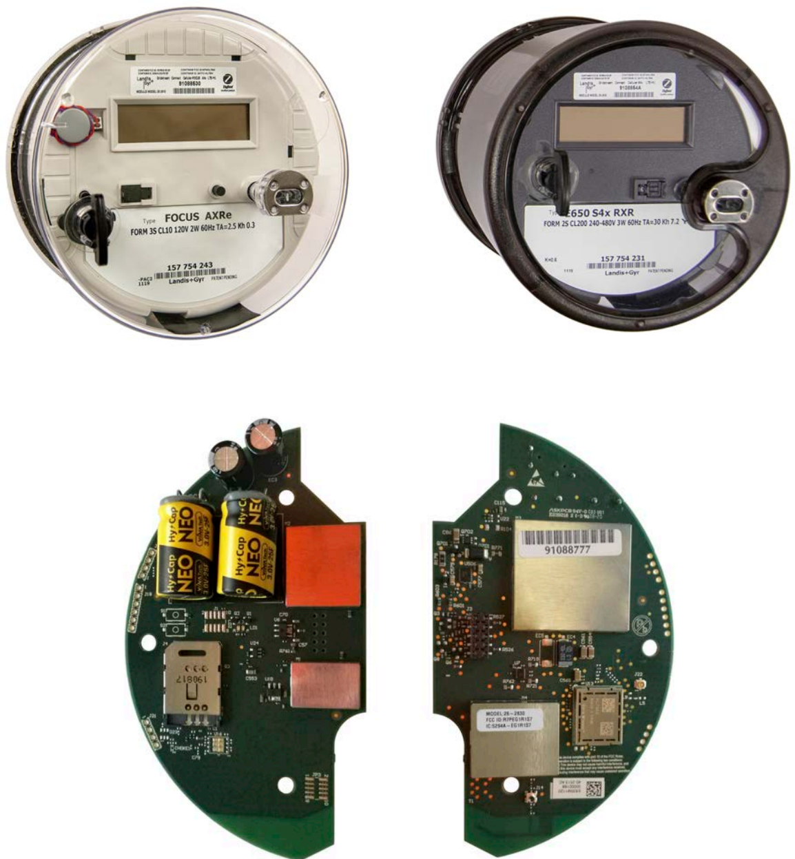
Figure 1. Landis+Gyr FOCUS AXe and S4x
