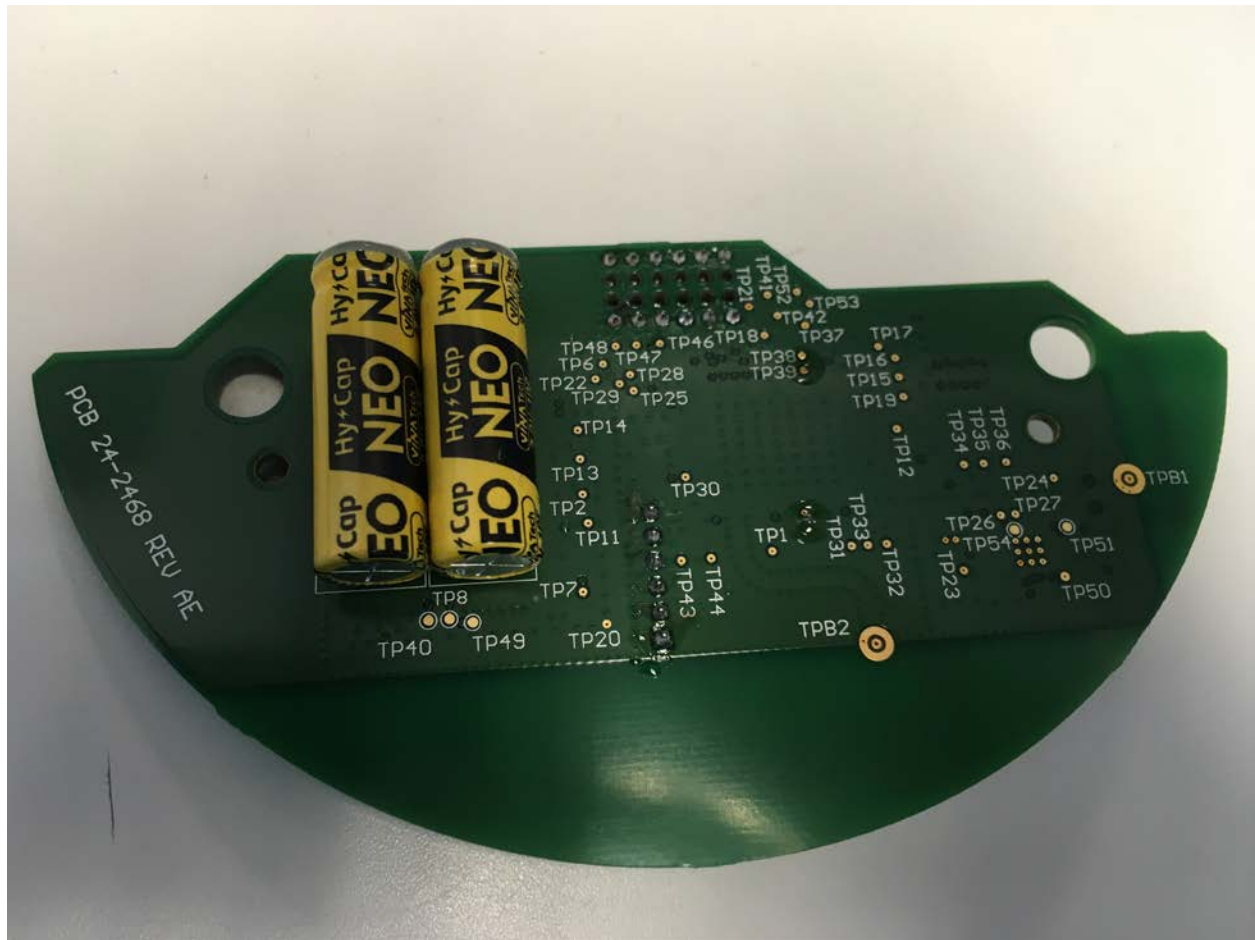
Figure 2: Bottom View
