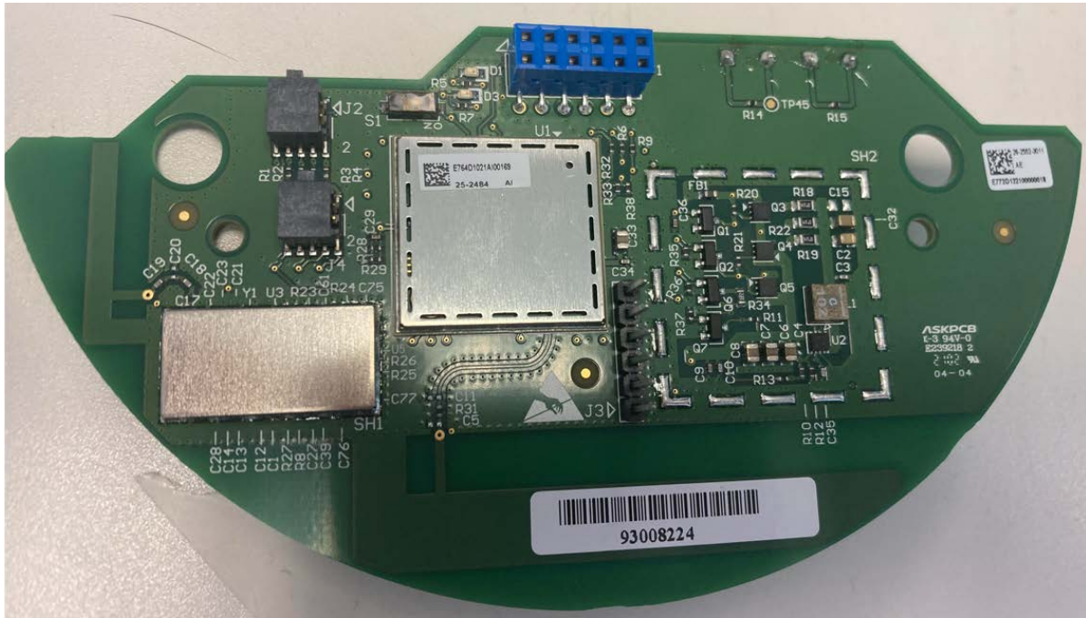
Figure 1: Top View
