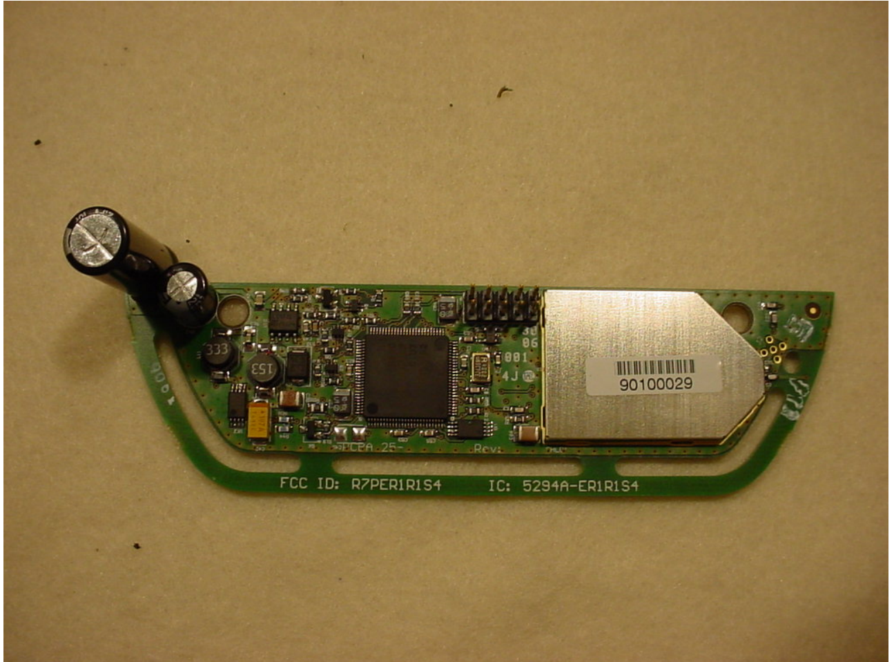
Figure 1: Internal - PCB Front Shielded
