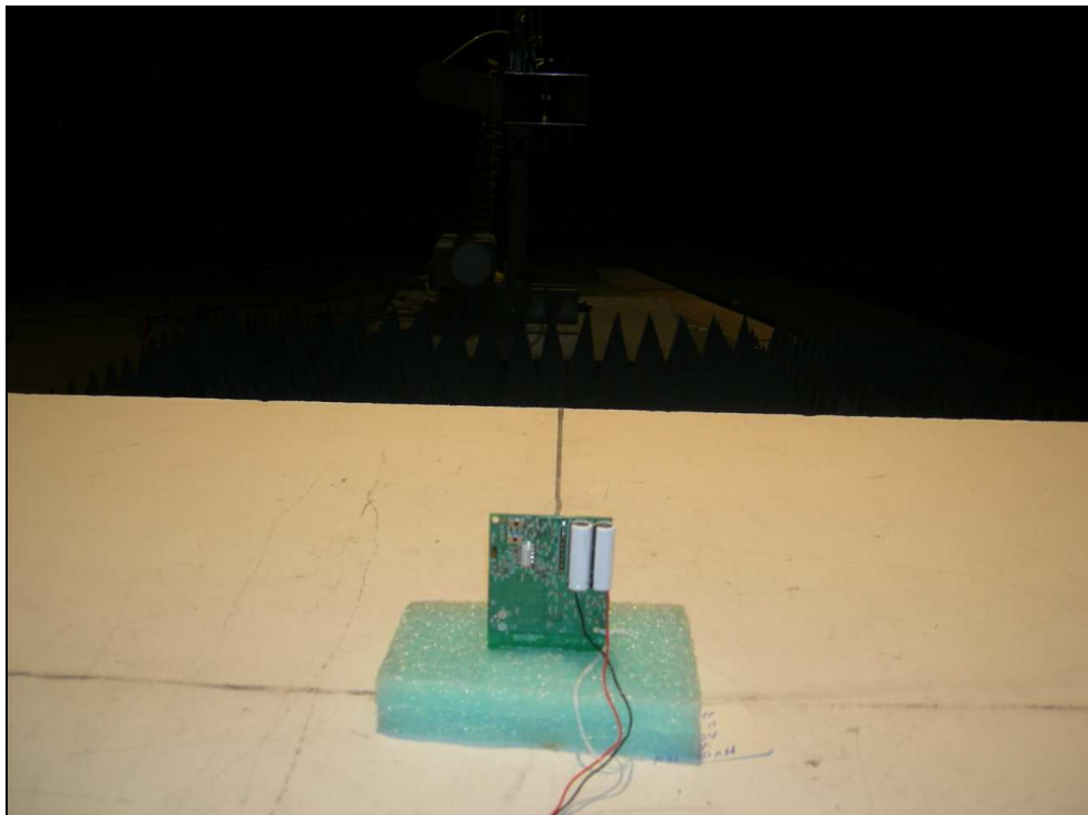
Figure 2: Test Setup Photo - Radiated Emissions
