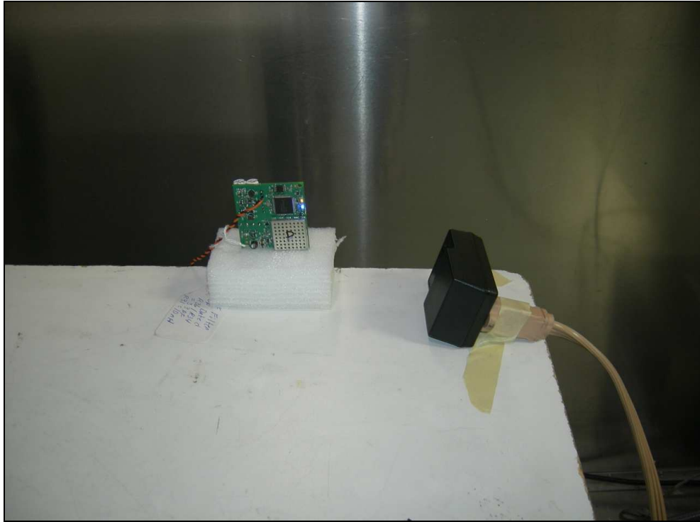
Figure 3: Test Setup Photo - Conducted Emissions
