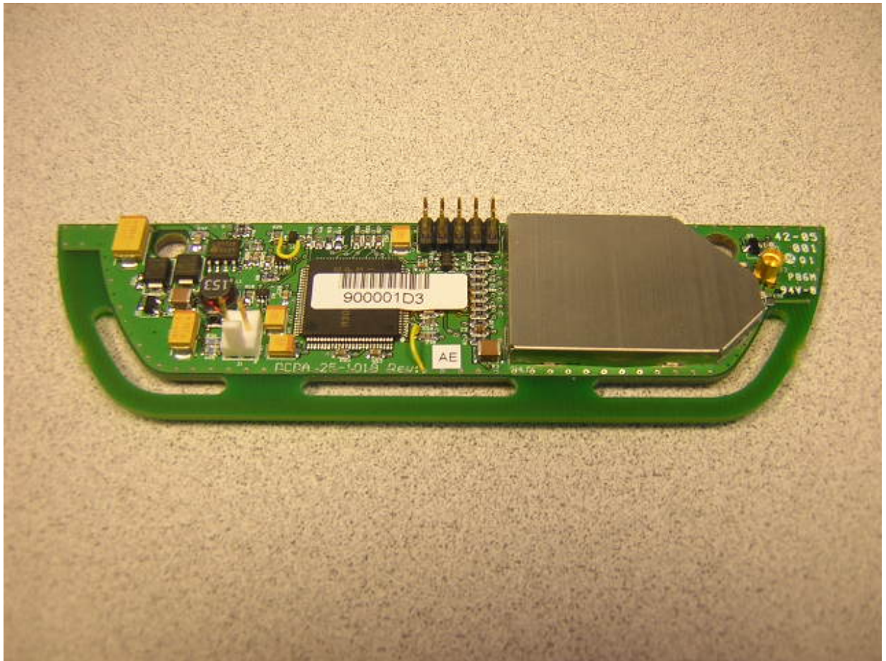
Figure 2: External – PCB Front With Shielding
