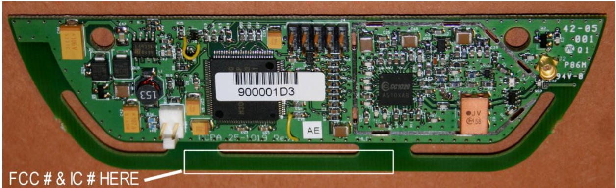
Figure 1: External – PCB Front Without Shielding
