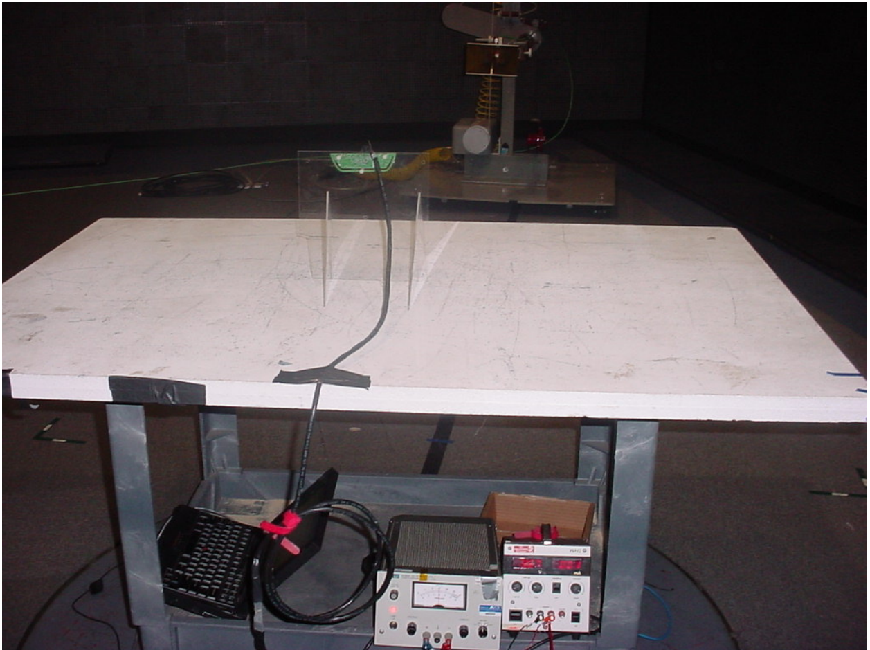
Figure 1: Test Setup - Radiated Emissions
