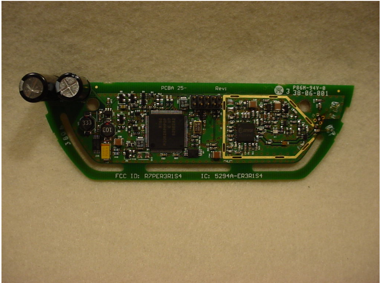
Figure 2: Internal - PCB Front No Shield
