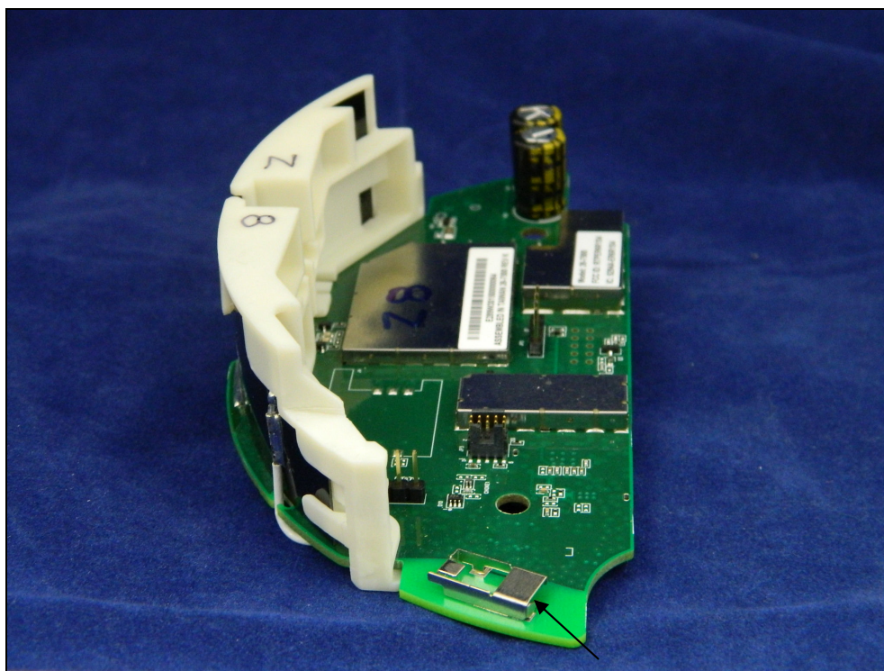
Figure 4: External Photo – Zigbee Antenna
