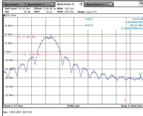
Figure 7.5.1.2-10: Upper Band-edge – Port 1
