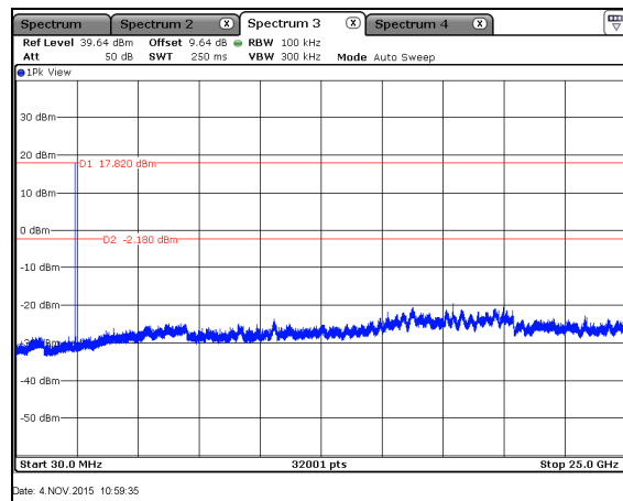
Figure 7.5.1.2-2: 30 MHz – 25 GHz – Port 0 MCH
