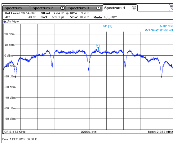
Figure 7.6.2-6: PSD Plot – HCH – Port 1
