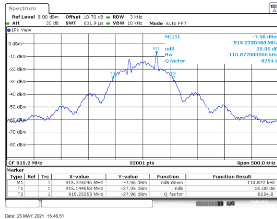
Figure 7.3.2-4: 20dB BW Mid Channel – 50kbps
