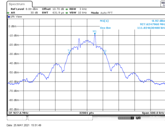
Figure 7.3.2-12: 99% BW High Channel – 50kbps
