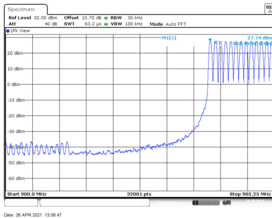
Figure 7.4.2.2-7: Mode 2 (239 Channels)
