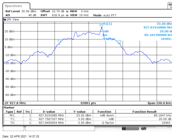
Figure 7.4.4.2-17: 20 dB BW Mid Channel – 38.4kbps
