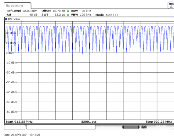
Figure 7.4.2.2-10: Mode 2 (239 Channels)
