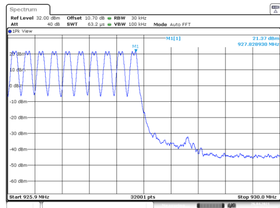
Figure 7.4.2.2-20: Mode 4 (129 Channels)
