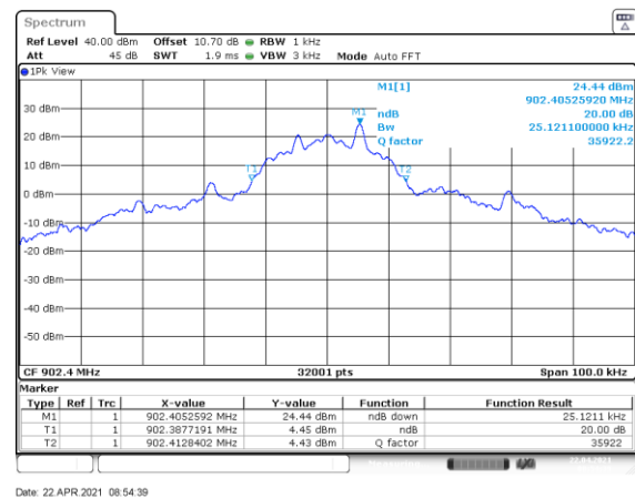
Figure 7.4.4.2-4: 20 dB BW Low Channel – 10kbps
