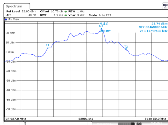
Figure 7.4.4.2-37 99% BW Mid Channel -50kbps
