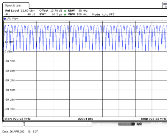
Figure 7.4.2.2-11: Mode 2 (86 Channels)
