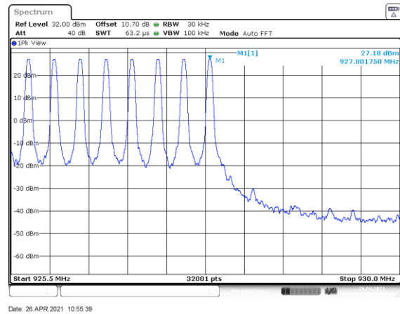
Figure 7.4.2.2-6: Mode 1 (86 Channels)
