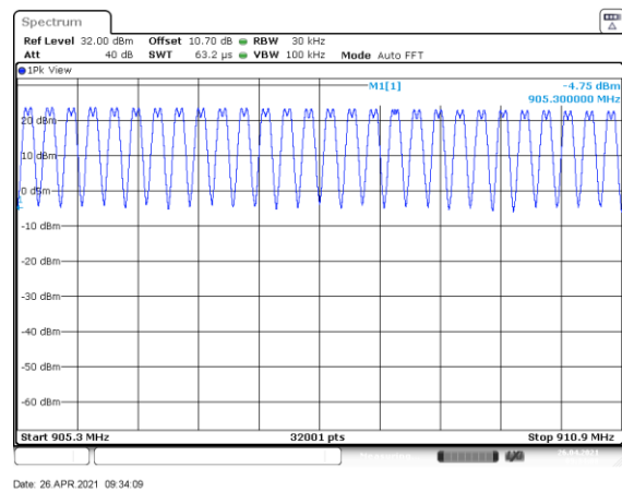
Figure 7.4.2.2-16: Mode 2 (129 Channels)
