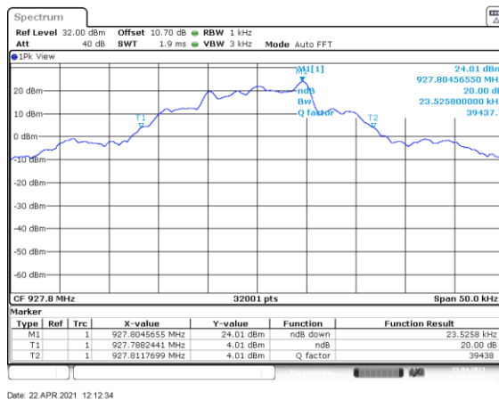
Figure 7.4.4.2-15: 20 dB BW High Channel – 9.6kbps
