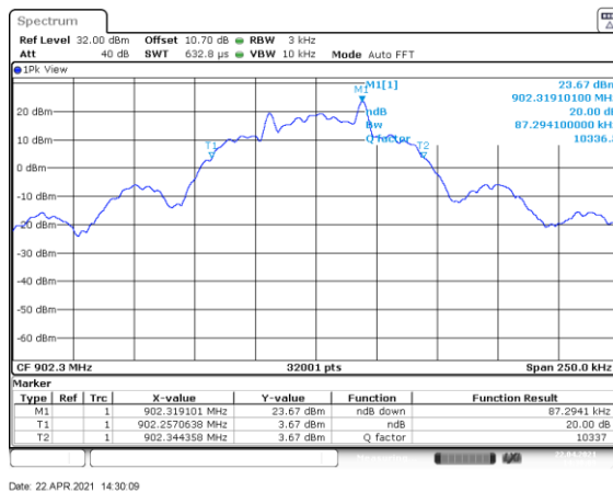
Figure 7.4.4.2-3: 20 dB BW Low Channel – 38.4kbps
