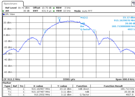
Figure 7.4.4.2-23: 20 dB BW Mid Channel -150kbps
