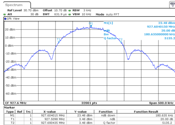
Figure 7.4.4.2-24: 20 dB BW High Channel -150kbps
