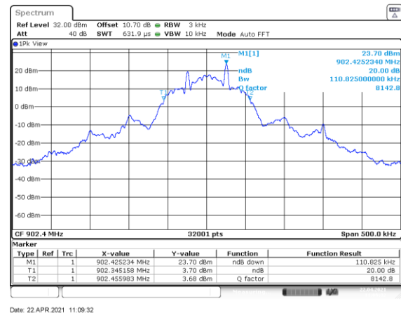
Figure 7.4.4.2-6: 20 dB BW Low Channel – 50kbps
