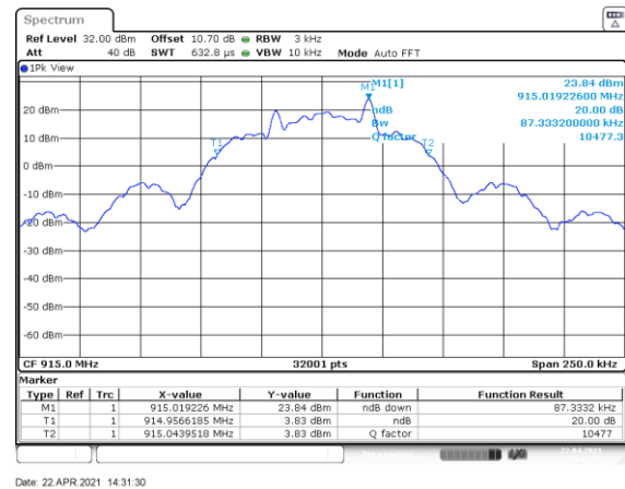
Figure 7.4.4.2-10: 20 dB BW Mid Channel – 38.4kbps
