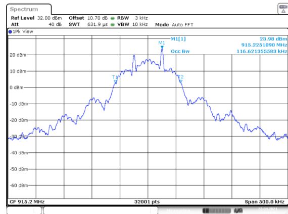
Figure 7.4.4.2-35: 99% BW Mid Channel -10kbps
