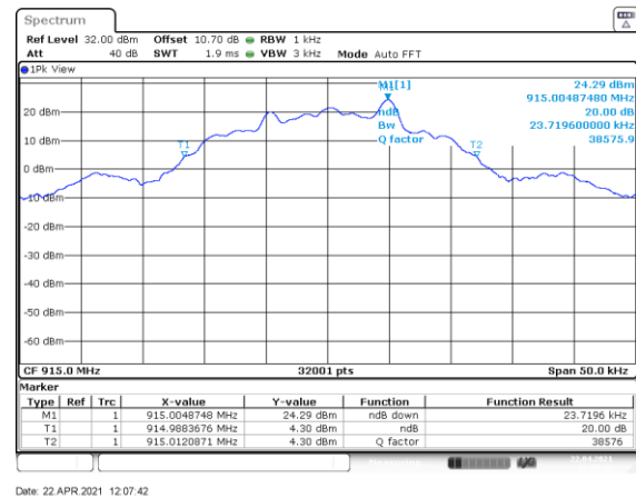
Figure 7.4.4.2-8: 20 dB BW Mid Channel – 9.6kbps
