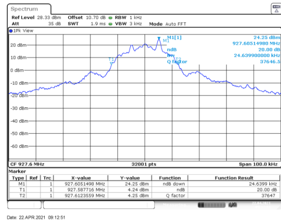
Figure 7.4.4.2-18: 20 dB BW Mid Channel – 10kbps
