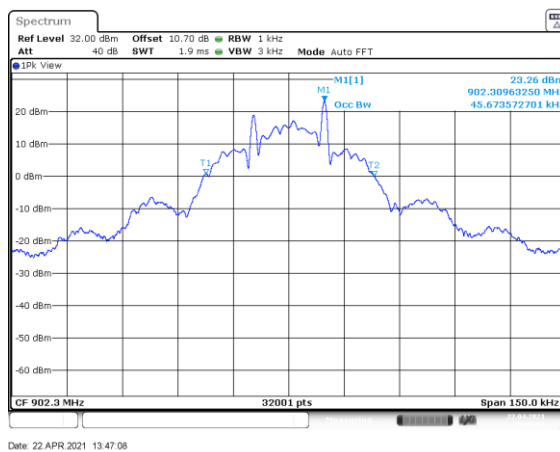
Figure 7.4.4.2-25: 99% BW Low Channel -19.2kbps
