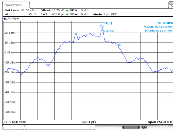
Figure 7.4.4.2-34: 99% BW Mid Channel -38.4kbps
