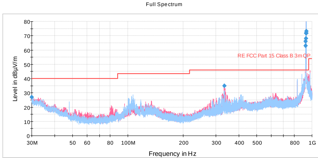
Figure A-3: Radiated Emissions – 30 MHz – 1 GHz
