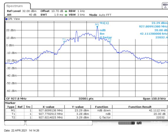
Figure 7.4.4.2-16: 20 dB BW High Channel – 19.2kbps
