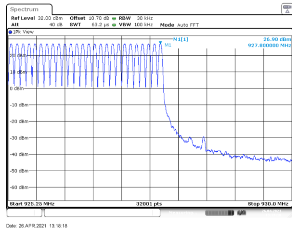
Figure 7.4.2.2-12: Mode 2 (86 Channels)
