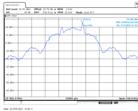
Figure 7.4.4.2-26: 99% BW Low Channel -38.4kbps
