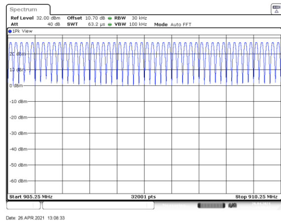
Figure 7.4.2.2-8: Mode 2 (239 Channels)
