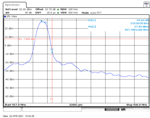
Figure 7.5.1.2-6: Upper Band edge – Mode 1
