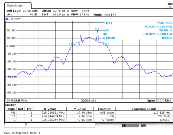
Figure 7.4.4.2-14: 20 dB BW Mid Channel – 50kbps
