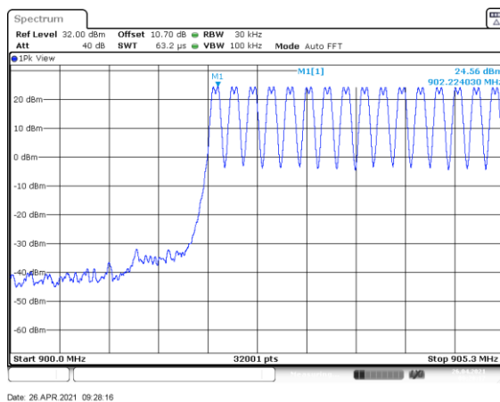
Figure 7.4.2.2-15: Mode 4 (129 Channels)
