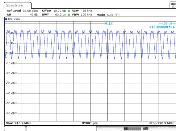
Figure 7.4.2.2-18: Mode 4 (129 Channels)
