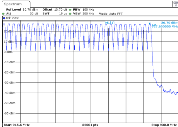
Figure 7.4.2.2-22: Mode 5 (64 Channels)
