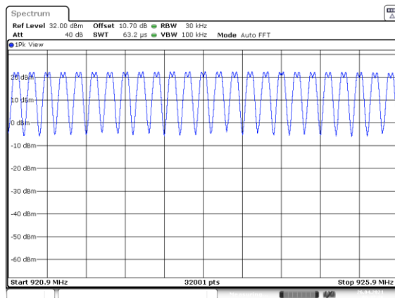
Figure 7.4.2.2-19: Mode 4 (129 Channels)
