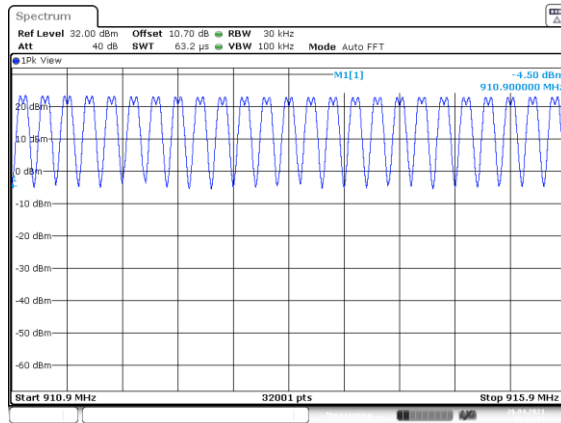
Figure 7.4.2.2-17: Mode 4 (129 Channels)
