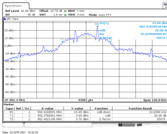
Figure 7.4.4.2-5: 20 dB BW Low Channel – 20kbps
