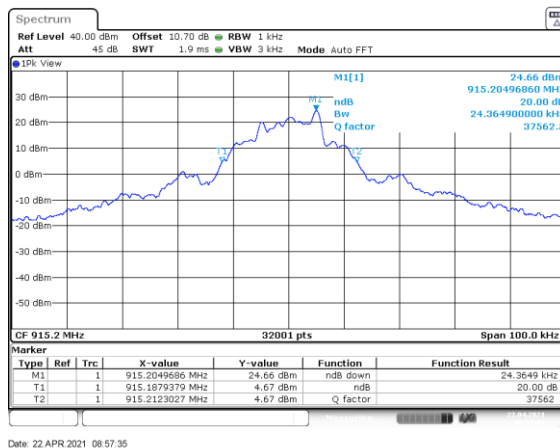
Figure 7.4.4.2-11: 20 dB BW Mid Channel – 10kbps
