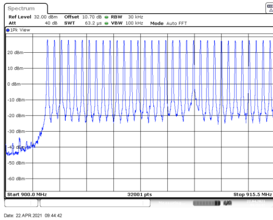
Figure 7.4.2.2-13: Mode 3 (64 Channels)
