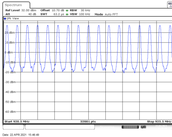
Figure 7.4.2.2-5: Mode 1 (86 Channels)
