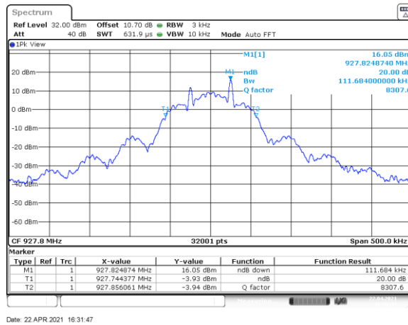
Figure 7.4.4.2-21: 20 dB BW High Channel – 50kbps
