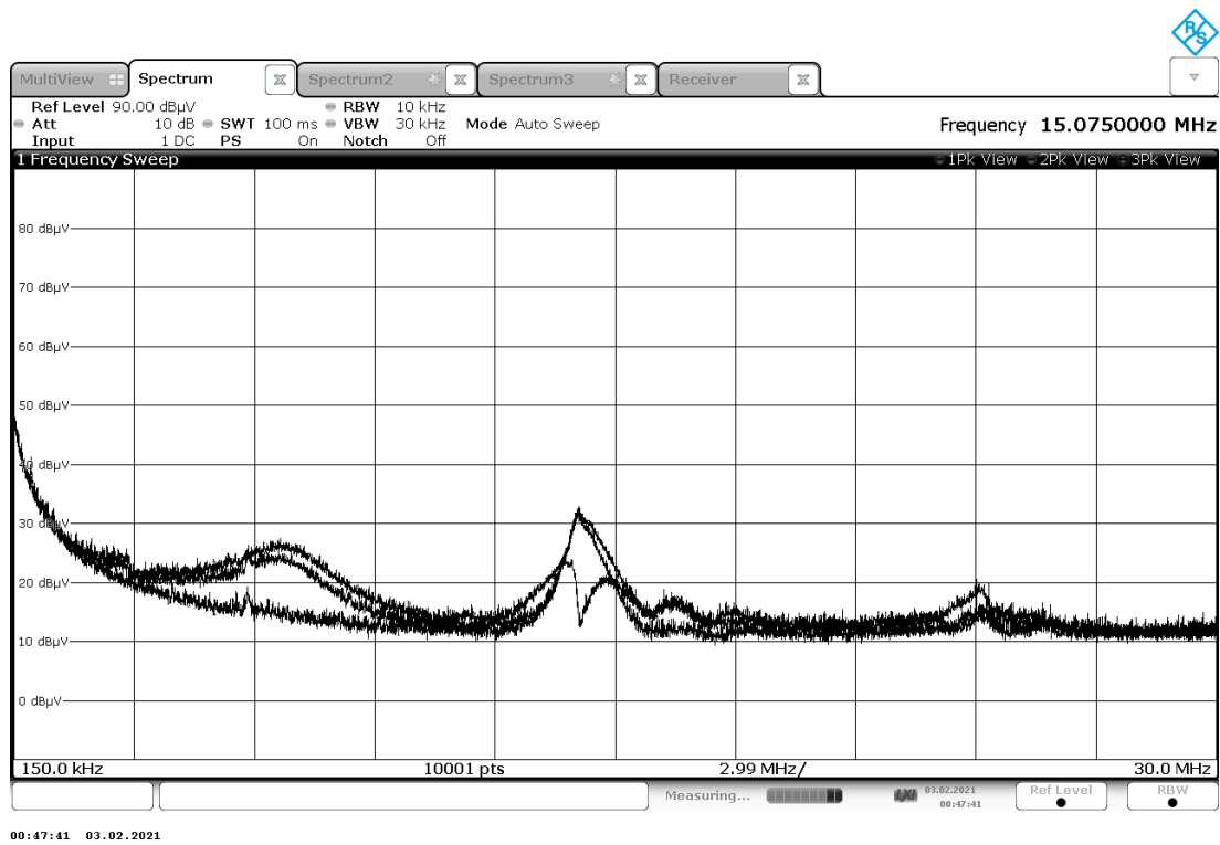
Figure A-2: Radiated Emissions – 150 kHz to 30 MHz
