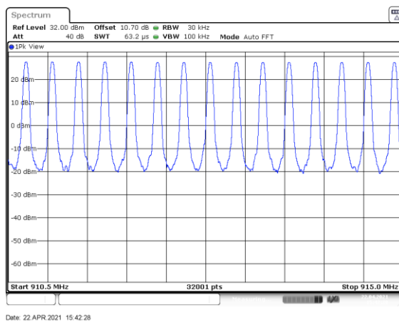
Figure 7.4.2.2-1: Mode 1 (86 Channels)
