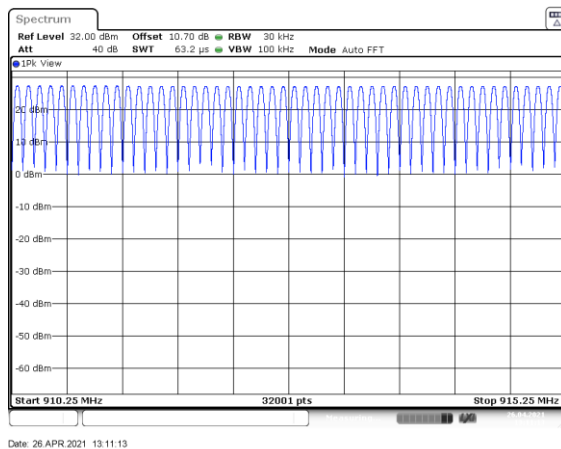
Figure 7.4.2.2-9: Mode 2 (239 Channels)
