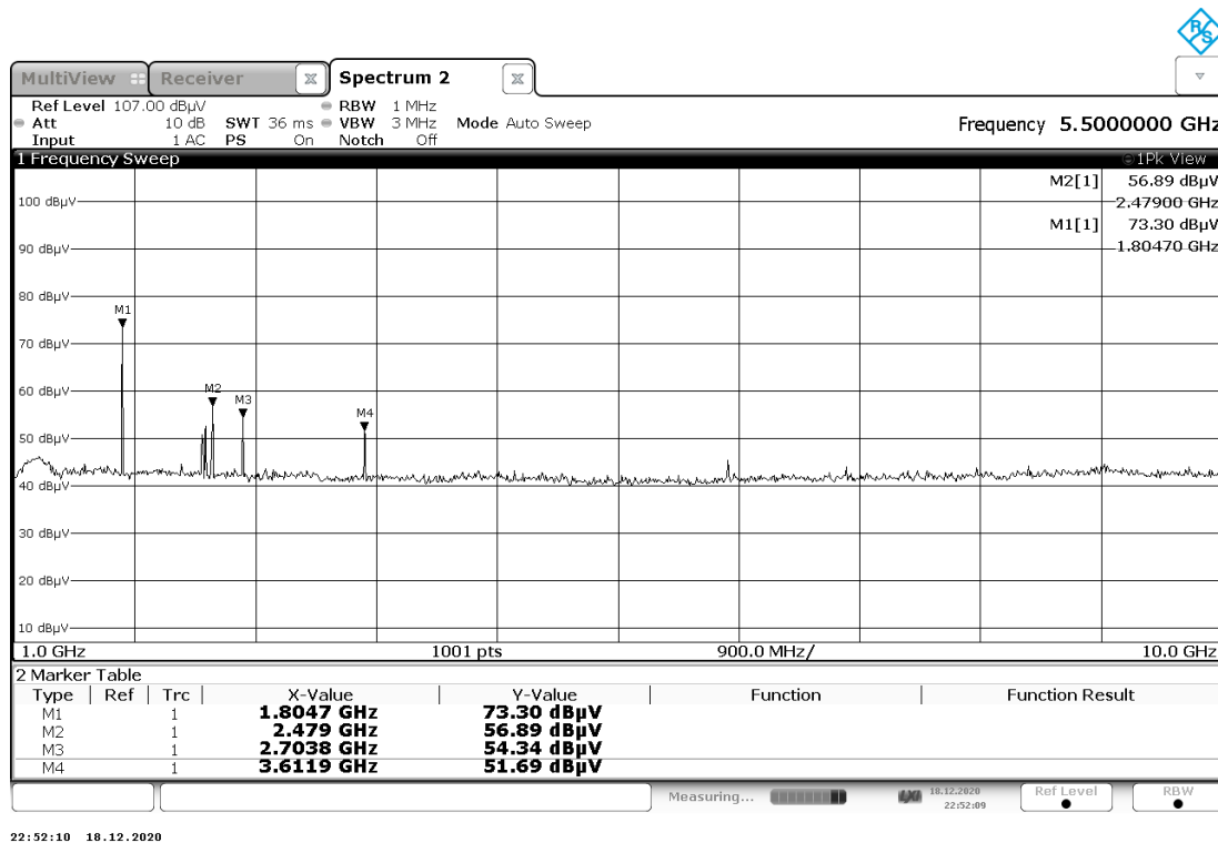
Figure A-4: Radiated Emissions – 1 GHz – 10 GHz
