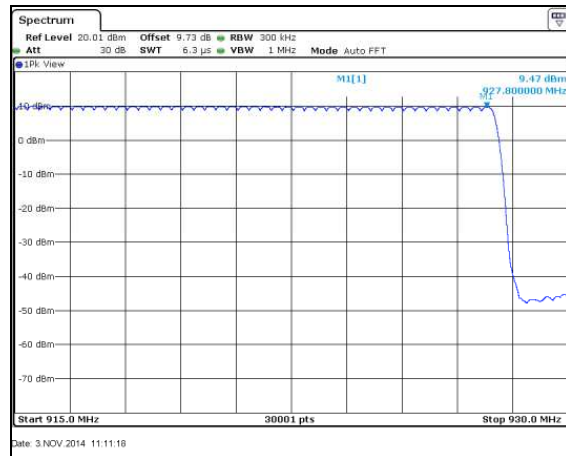
Figure 7.4.2.2-2: Mode 1 (86 Channels)
