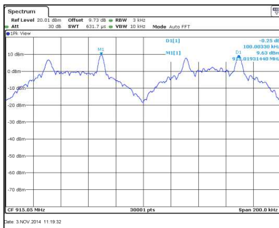
Figure 7.4.1.2-2: Mode 2
