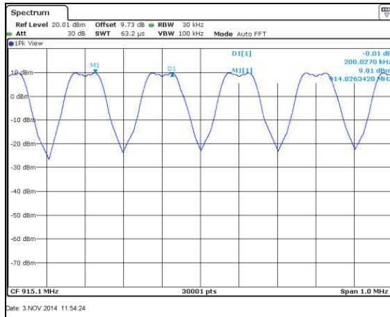
Figure 7.4.1.2-4: Mode 4
