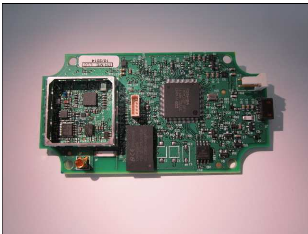
Figure 4: Internal Photo (without shields)
