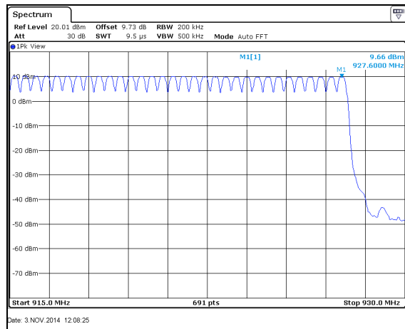
Figure 7.4.2.2-14: Mode 5 (64 Channels)
