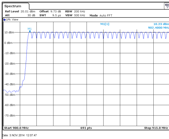
Figure 7.4.2.2-13: Mode 5 (64 Channels)
