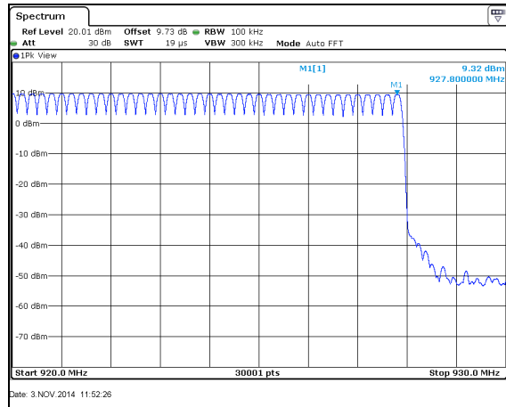
Figure 7.4.2.2-12: Mode 4 (129 Channels)
