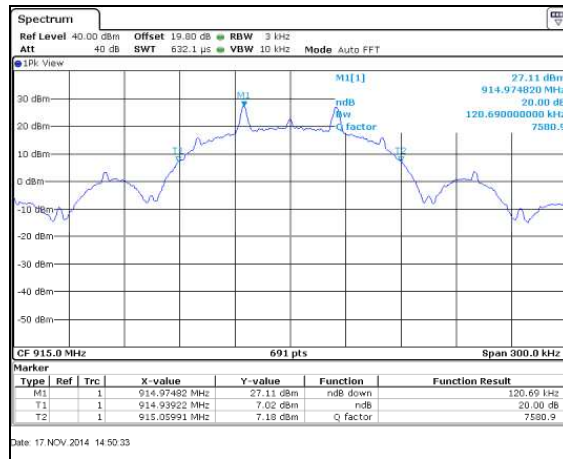
Figure 7.4.4.2-4: 20dB BW Mid Channel - 50.0kbps
