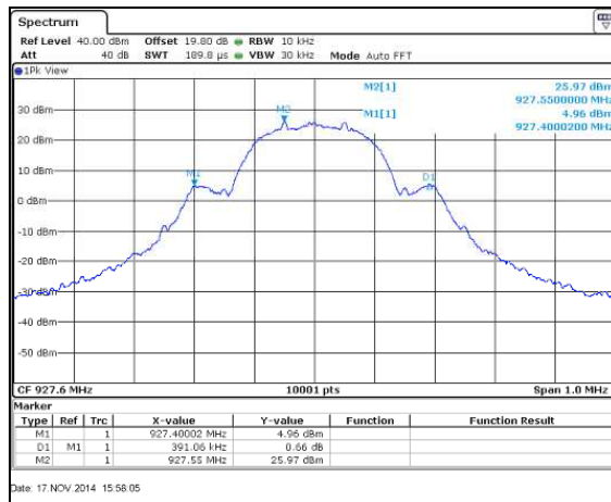
Figure 7.4.4.2-9: 20dB BW High Channel – 200.0kbps
