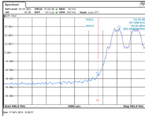
Figure 7.5.1.2-6: Lower Band-edge – Mode 5
