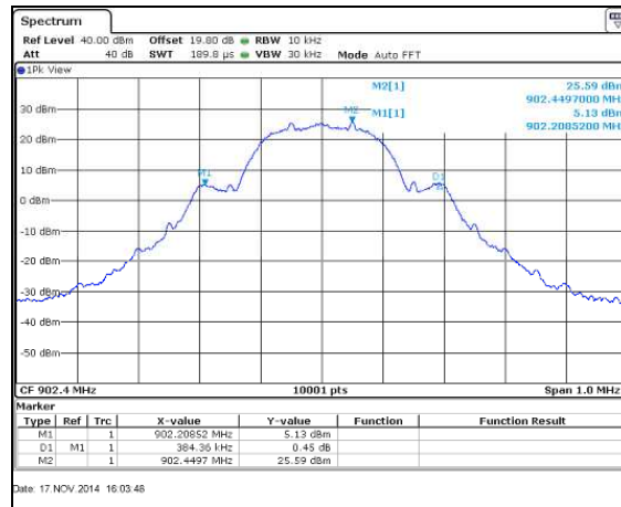
Figure 7.4.4.2-3: 20dB BW Low Channel - 200.0kbps
