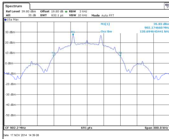
Figure 7.4.4.2-10: 99% BW Low Channel – 50.0kbps
