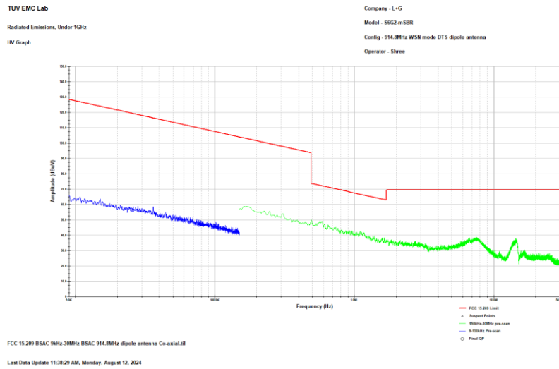
Figure 1: Reference plot for Radiated Spurious Emissions – 9 kHz – 30 MHz- Co-axial – Mode 3 – MCH – Dipole Antenna
