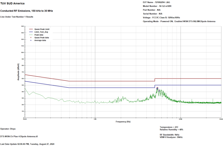
Figure 2.2.6-1: Conducted Emission Plot – Line 1 – Dipole Antenna
