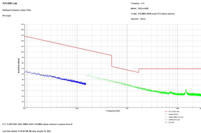
Figure 2: Reference plot for Radiated Spurious Emissions – 9 kHz – 30 MHz- Co-Planar Horz. – Mode 3 – MCH – Dipole Antenna
