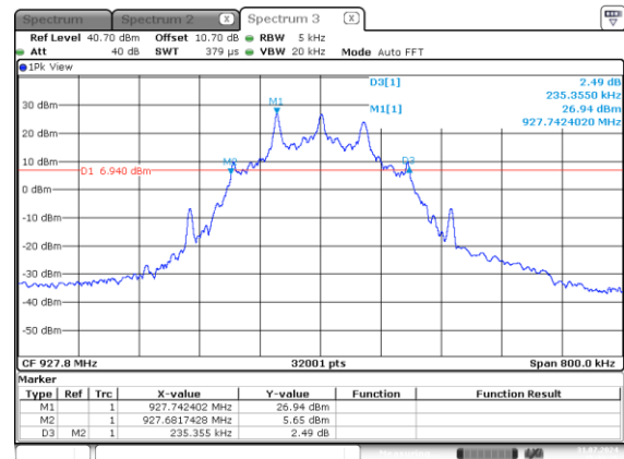
Figure 2.8.6-18: Mode 7 – 20 dB BW – HCH – 115.2 kbps
