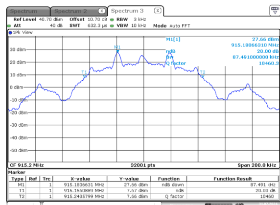
Figure 2.8.6-14: Mode 7 – 20 dB BW – MCH – 38.4 kbps
