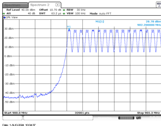
Figure 2.6.6-1: Mode 2 – 50 kbps (129 Channels)
