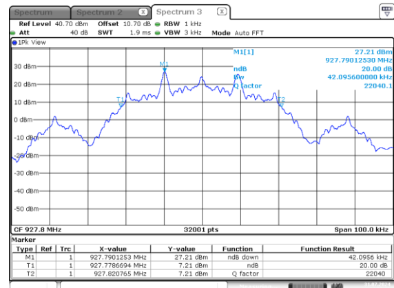
Figure 2.8.6-12: Mode 7 – 20 dB BW – HCH – 19.2 kbps
