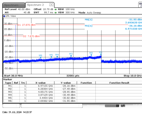
Figure 2.11.6-7:30MHz – 10GHz – LCH – Mode 7 – 9.6kbps Figure 2.11.6-8:30MHz – 10GHz – MCH – Mode 7 – 9.6kbps
