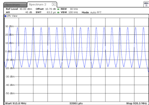
Figure 2.6.6-14: Mode 7 – 9.6 kbps (86 Channels)
