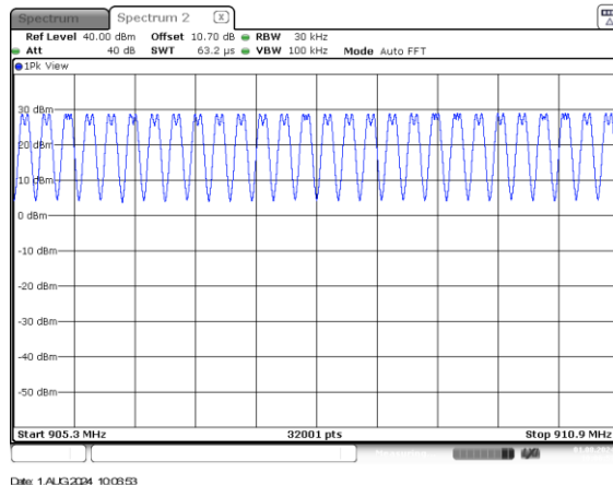
Figure 2.6.6-2: Mode 2 – 50 kbps (129 Channels)
