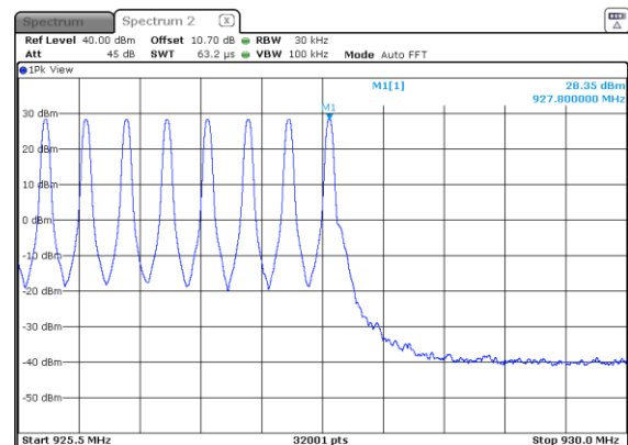
Figure 2.6.6-16: Mode 7 – 9.6 kbps (86 Channels)
