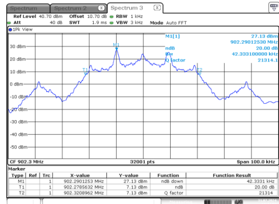
Figure 2.8.6-10: Mode 7 – 20 dB BW – LCH – 19.2 kbps
