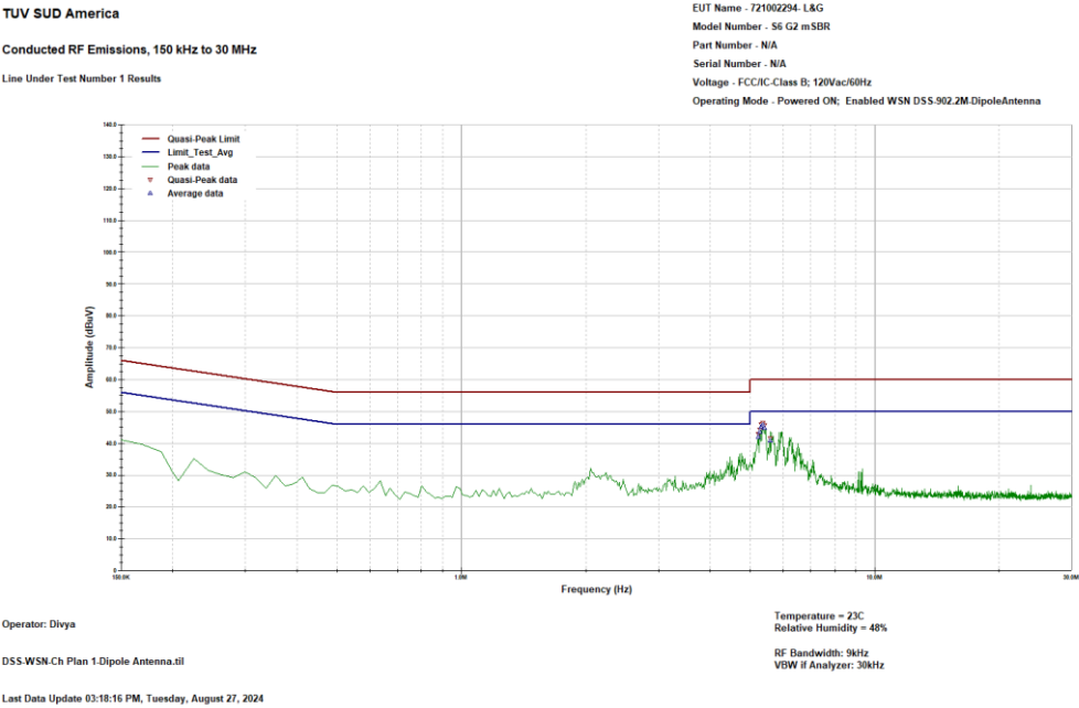
Figure 2.2.6-1: Conducted Emission Plot – Line 1 – Dipole Antenna
