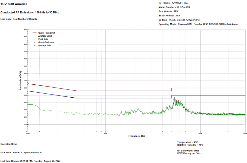
Figure 2.2.6-2: Conducted Emission Plot – Neutral -- Dipole Antenna
