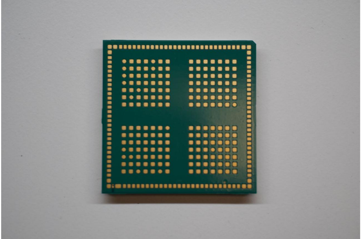
Figure 2: PCB Back
