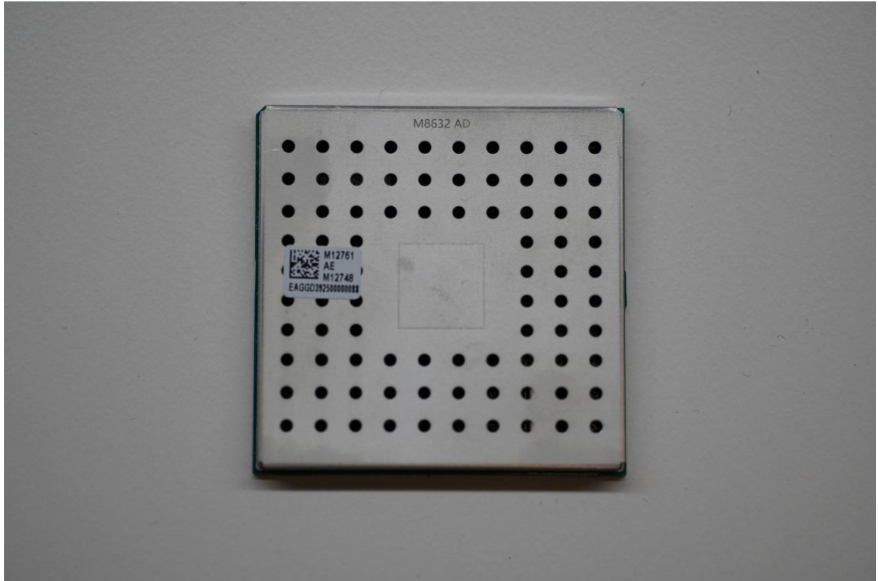
Figure 1: PCB Front
