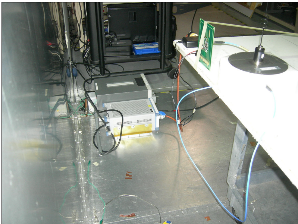
Figure 8: Conducted Emissions
