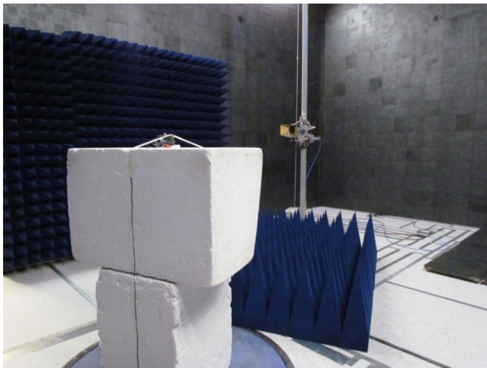
Figure 4: Equipment Under Test – Radiated Emissions – 1-10GHz
