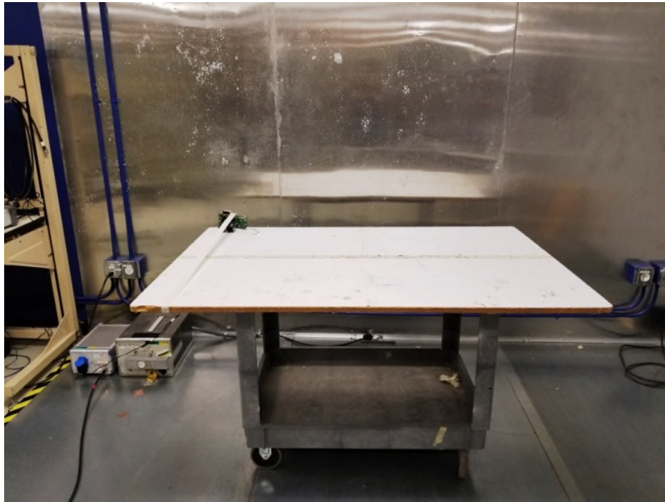
Figure 5: Equipment Under Test – AC Conducted Emissions
