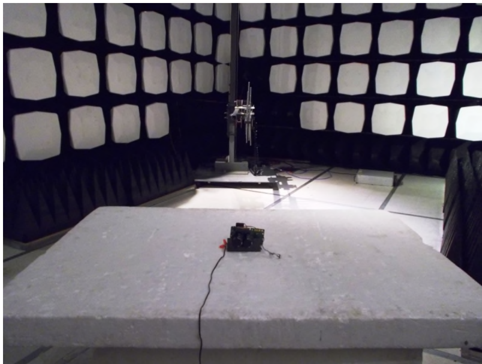
Figure 2: Equipment Under Test – Radiated Emissions – 30-1000MHz
