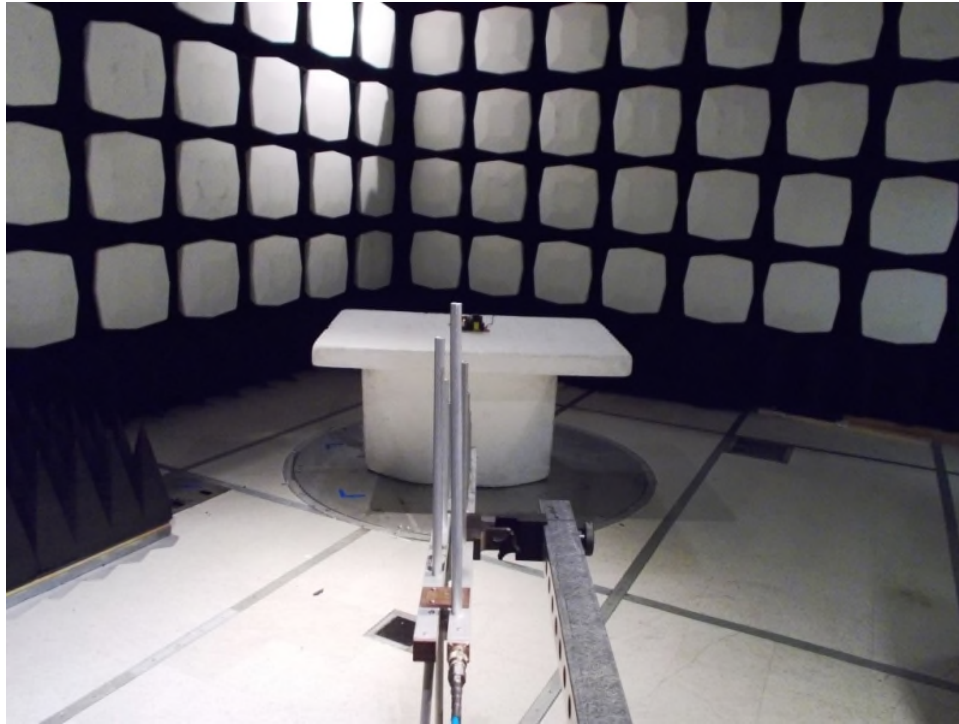
Figure 1: Equipment Under Test – Radiated Emissions – 30-1000MHz
