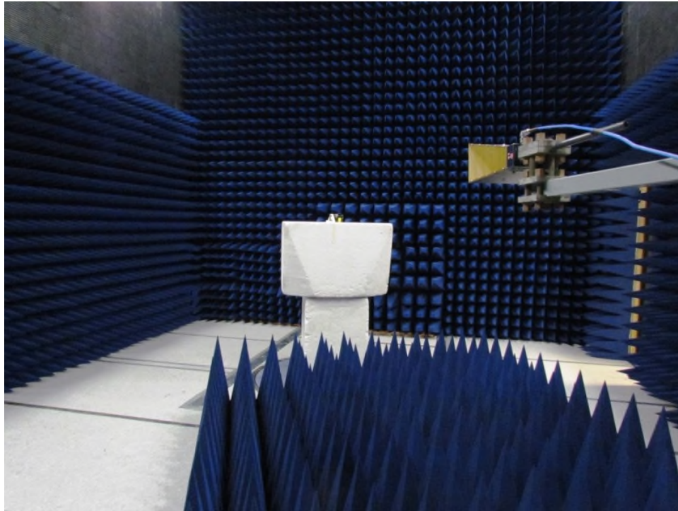
Figure 3: Equipment Under Test – Radiated Emissions – 1-10GHz
