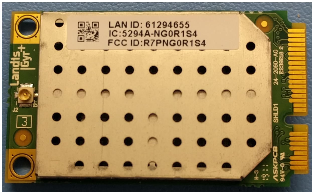
Figure 1: Top View
