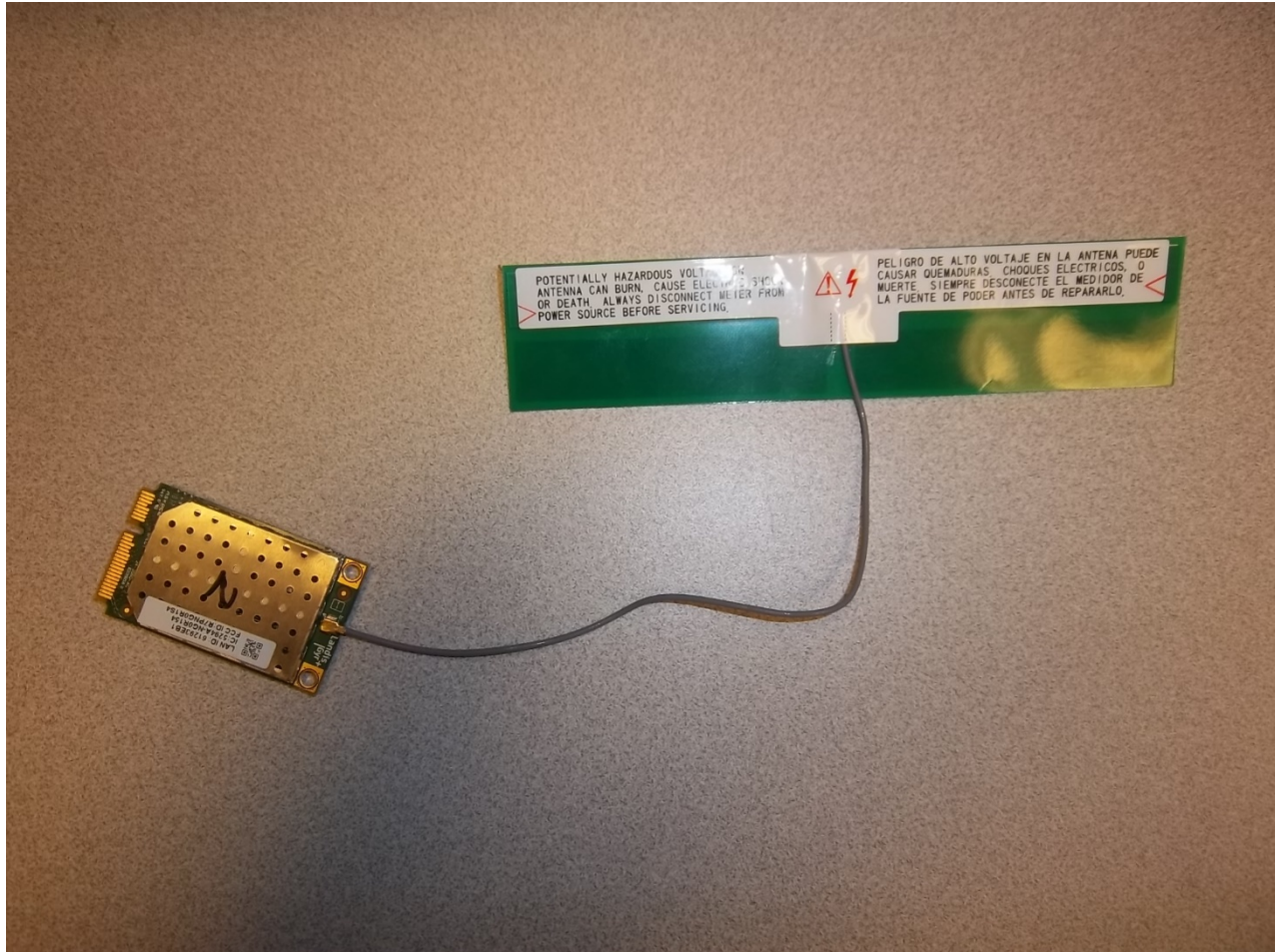
Figure 1: New Antenna.
