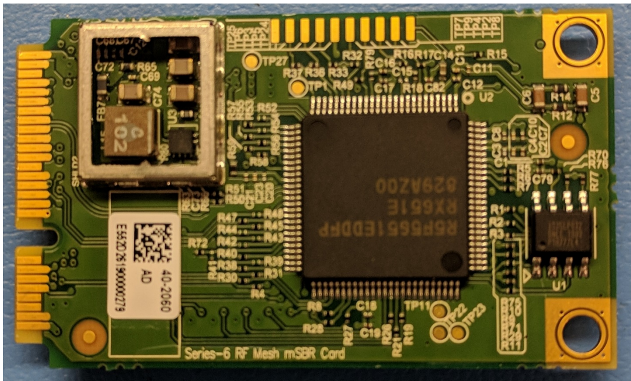
Figure 2: Bottom View
