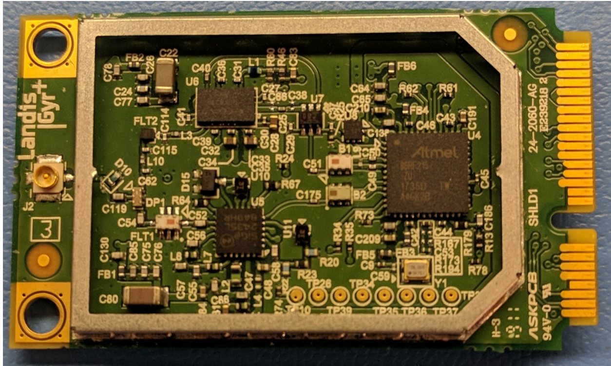
Figure 1: Top View
