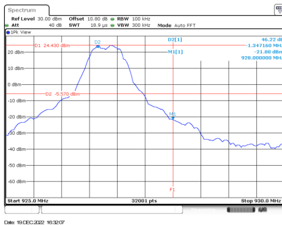
Figure 2.6.6-4: Upper Band edge – Mode 3 – MCS3
