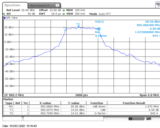
Figure 2.4.6-1: Mode 2 – 6 dB BW – LCH – MCS5
