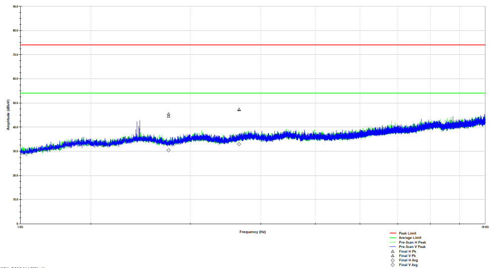
Figure 4: Reference plot for Radiated Spurious Emissions – 1.5 GHz – 10 GHz – Mode 3 – MCH – Dipole Antenna
