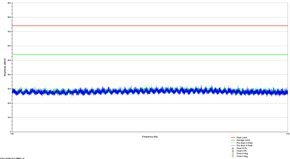
Figure 3: Reference plot for Radiated Spurious Emissions – 1 GHz – 1.5 GHz – Mode 3 – MCH – Dipole Antenna
