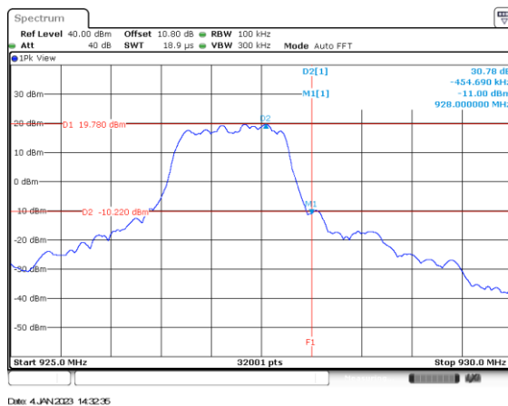
Figure 2.6.6-2: Upper Band edge – Mode 2 – MCS5
