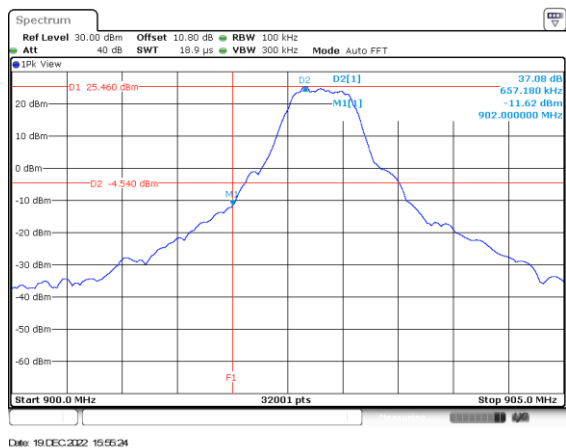
Figure 2.6.6-3: Lower Band edge – Mode 3 – MCS3
