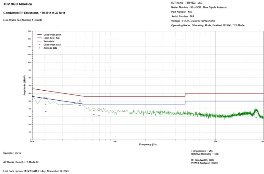
Figure 1: Conducted Emission Plot – Line 1
