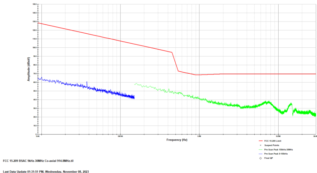
Figure 1: Reference plot for Radiated Spurious Emissions – 9 kHz – 30 MHz – Mode 1 – LCH
