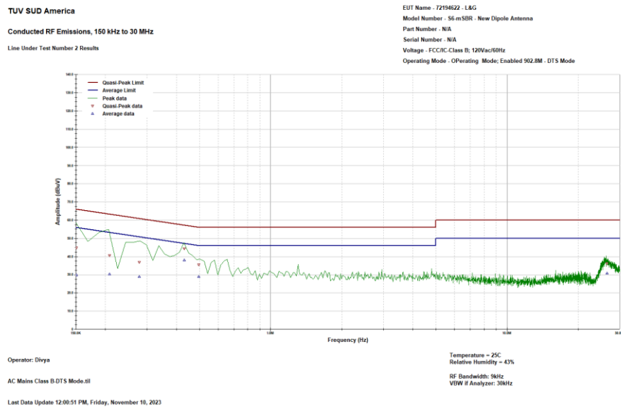
Figure 2: Conducted Emission Plot – Neutral
