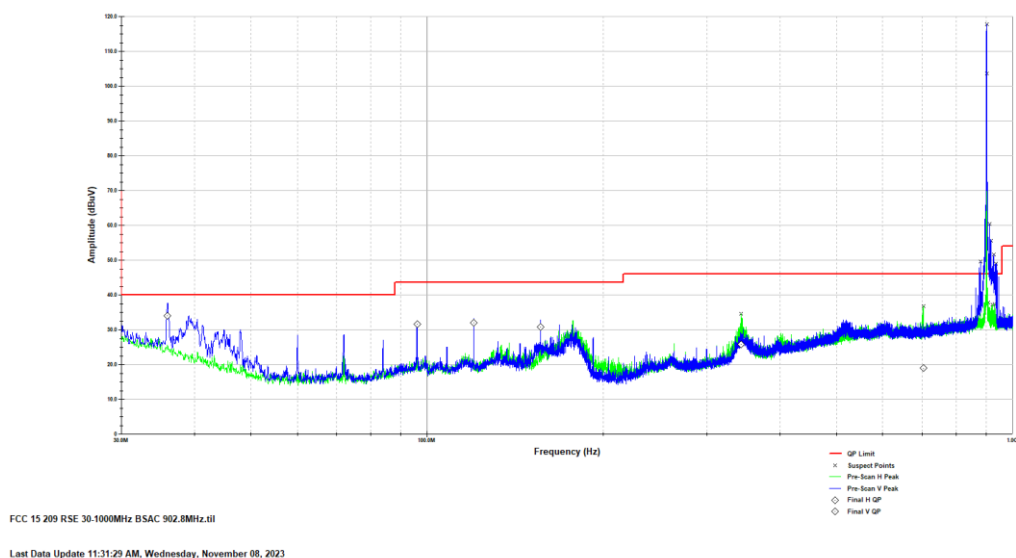
Figure 2: Reference plot for Radiated Spurious Emissions – 30 MHz – 1 GHz – Mode 1 – LCH
