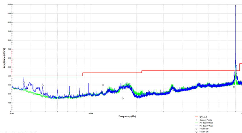
Figure 2: Reference plot for Radiated Spurious Emissions – 30 MHz – 1 GHz – Mode 1 – LCH - Dipole Antenna
