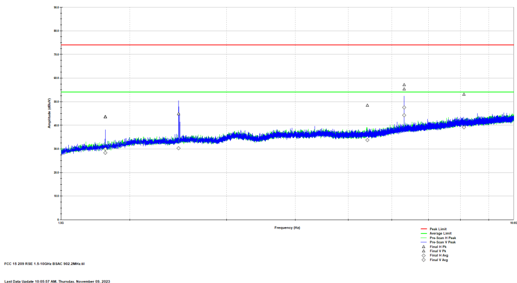
Figure 4: Reference plot for Radiated Spurious Emissions – 1.5 GHz – 10 GHz – Mode 1 – LCH – Dipole Antenna
