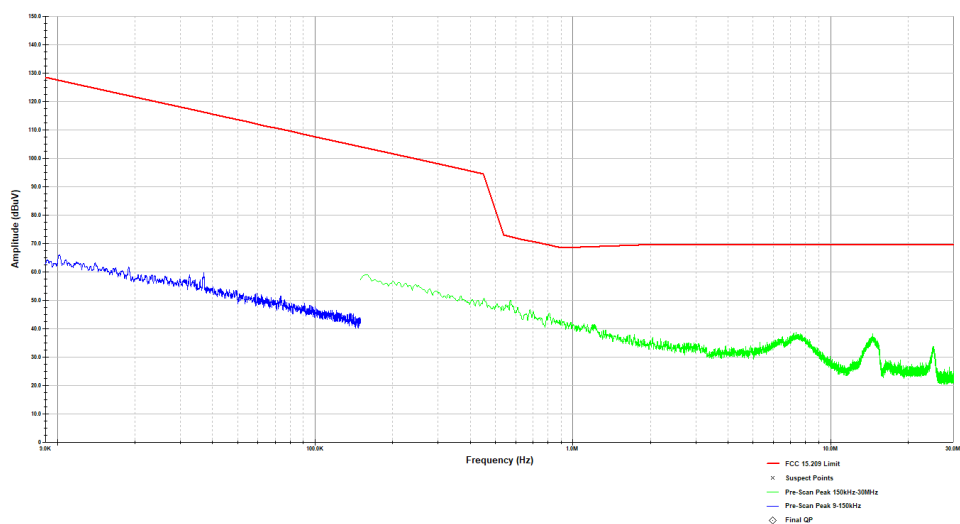
Figure 1: Reference plot for Radiated Spurious Emissions – 9 kHz – 30 MHz – Mode 1 – LCH – Dipole Antenna
