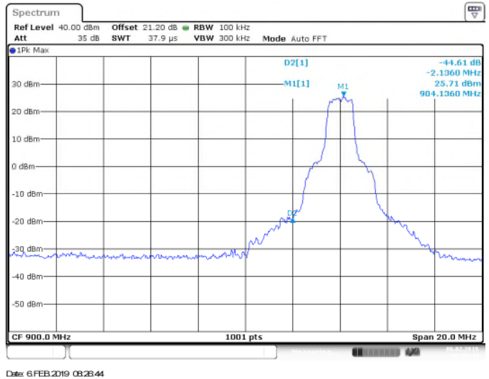
Figure 7.5.1.2-4: Lower Band-edge
