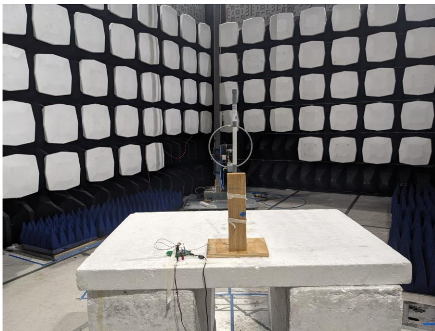
Figure2 – Rear View Test Set up - Radiated Emissions <30 MHz
