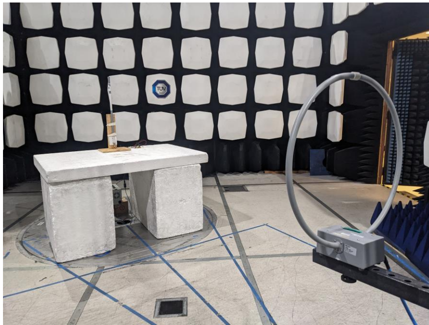
Figure1 – Front View Test Set up - Radiated Emissions <30 MHz
