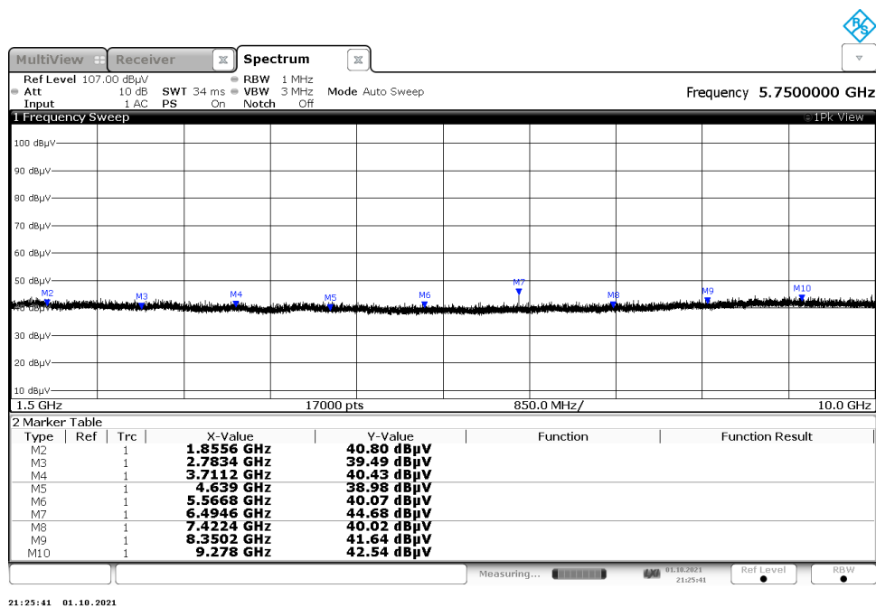
Figure 5: Reference plot for Radiated Spurious Emissions – 1.5 GHz – 10 GHz – Mode 2 Note: Emissions above the noise floor do not falls within restricted bands.
