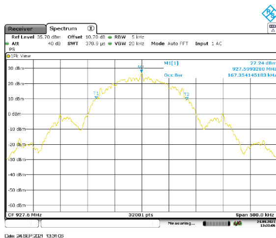
Figure 2.8.6-21: Mode 1 – 99% BW – HCH - 150 kbps
