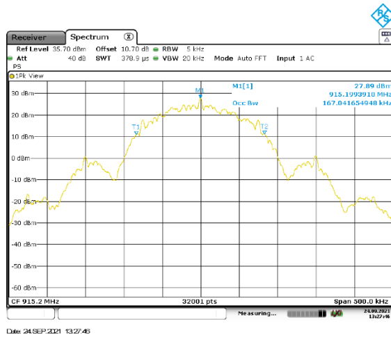
Figure 2.8.6-17: Mode 1 – 99% BW – MCH - 150 kbps
