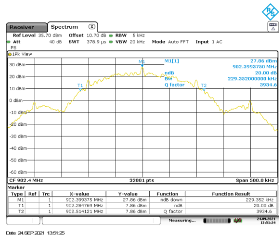
Figure 2.8.6-2: Mode 1 – 20 dB BW – LCH - 200 kbps
