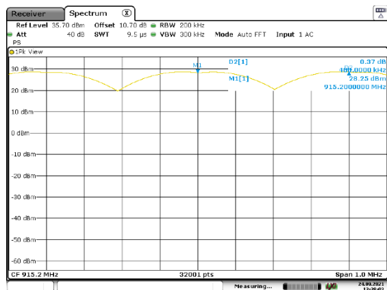
Figure 2.5.6-1: Channel Separation – Mode 1 – 150kbps
