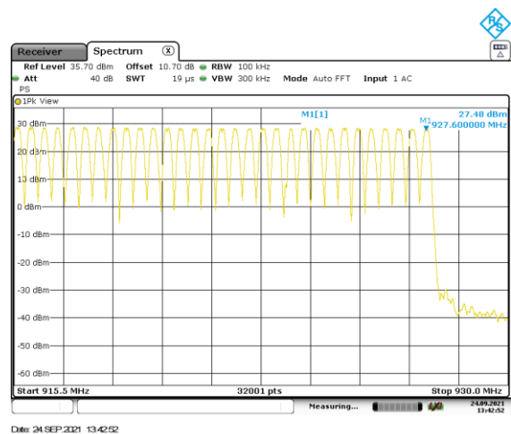
Figure 2.6.6-2: Mode 1 – 150 kbps (64 Channels)
