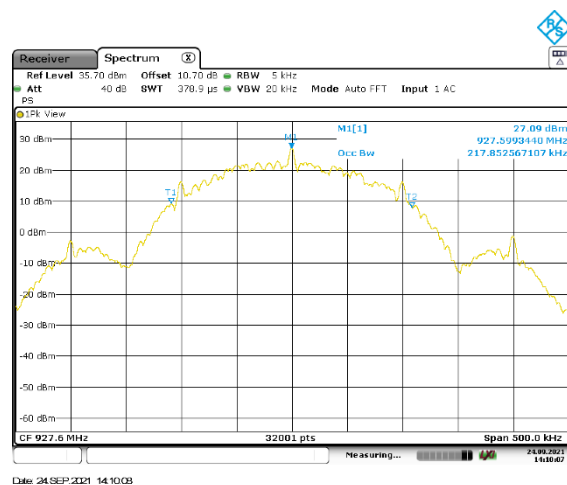
Figure 2.8.6-22: Mode 1 – 99% BW – HCH -200kbps
