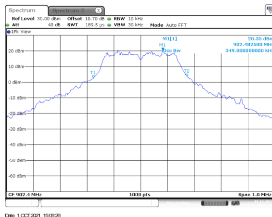
Figure 2.8.6-16: Mode 5 – 99% BW – LCH – MCS2
