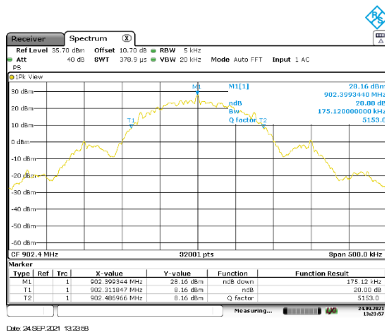
Figure 2.8.6-1: Mode 1 – 20 dB BW – LCH - 150 kbps
