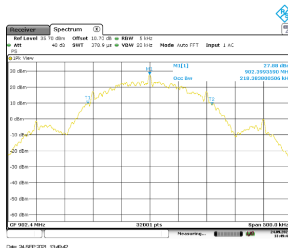
Figure 2.8.6-12: Mode 5 – 20 dB BW – HCH – MCS2
