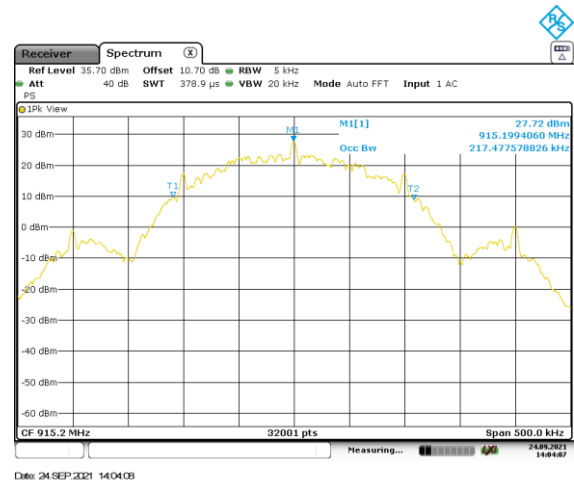
Figure 2.8.6-18: Mode 1 – 99% BW – MCH – 200kbps
