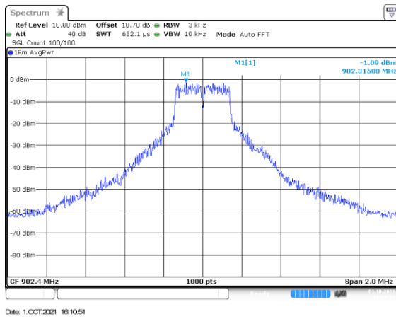
Figure 2.9.6-1: Mode 5 – PSD – LCH – MCS2
