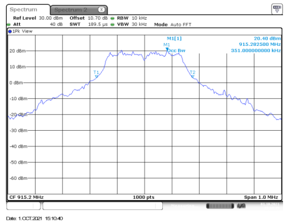
Figure 2.8.6-20: Mode 5 – 99% BW – MCH – MCS2
