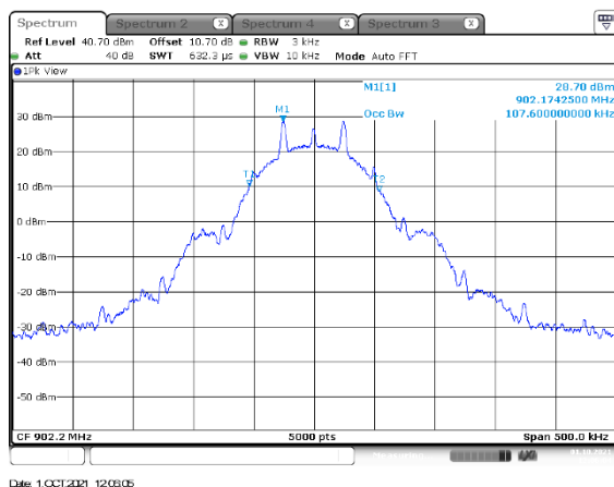
Figure 2.8.6-15: Mode 2 – 99 % BW – LCH - 50 kbps
