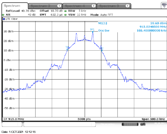
Figure 2.8.6-19: Mode 2 – 99% BW – MCH - 50 kbps
