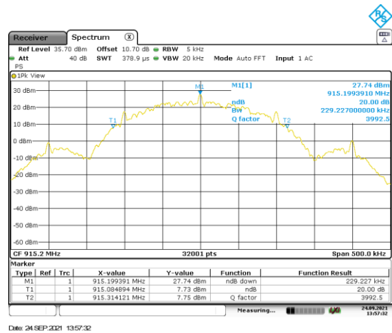
Figure 2.8.6-6: Mode 1 – 20 dB BW – MCH –200kbps
