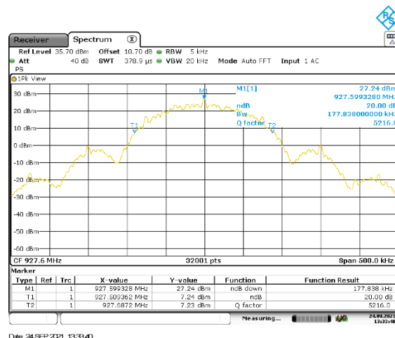
Figure 2.8.6-9: Mode 1 – 20 dB BW – HCH - 150 kbps
