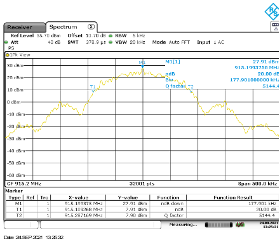
Figure 2.8.6-5: Mode 1 – 20 dB BW – MCH - 150 kbps
