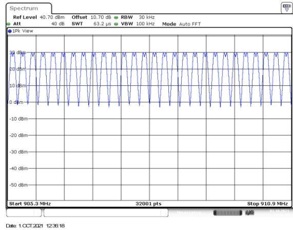
Figure 2.6.6-4: Mode 2 – 50 kbps (129 Channels)
