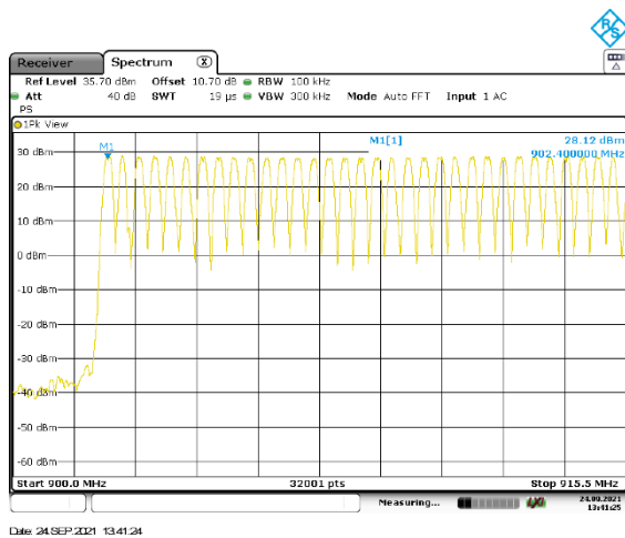
Figure 2.6.6-1: Mode 1 – 150 kbps (64 Channels)
