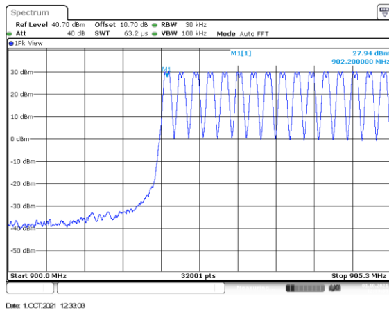
Figure 2.6.6-3: Mode 2 – 50 kbps (129 Channels)
