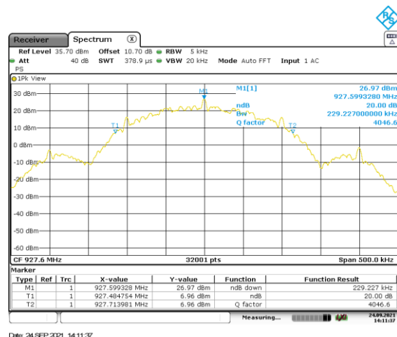
Figure 2.8.6-10: Mode 1 – 20 dB BW – HCH – 200 kbps
