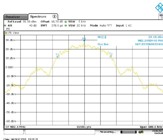
Figure 2.8.6-11: Mode 2 – 20 dB BW – HCH - 50 kbps
