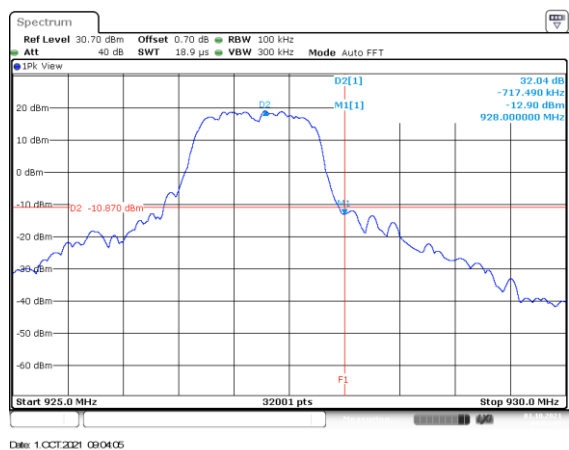
Figure 2.6.6-4: Higher Band edge – Mode 2 – MCS5
