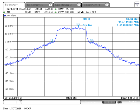
Figure 2.4.6-18: Mode 2 – 99% BW – MCH - MCS5
