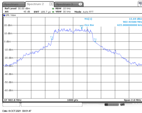
Figure 2.4.6-15: Mode 3 – 99% BW – LCH – MCS3
