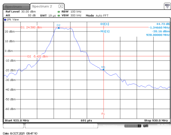
Figure 2.6.6-6: Higher Band edge – Mode 3 – MCS3
