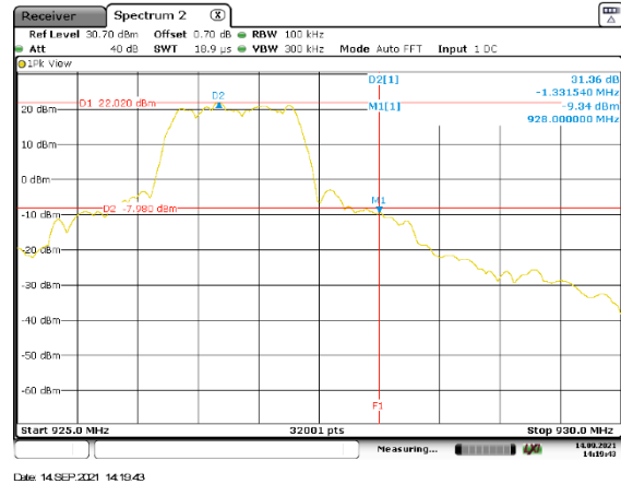
Figure 2.6.6-2: Higher Band edge – Mode 1 – MCS0
