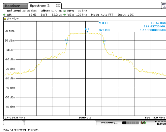
Figure 2.4.6-17: Mode 1 – 99% BW – MCH – MCS0
