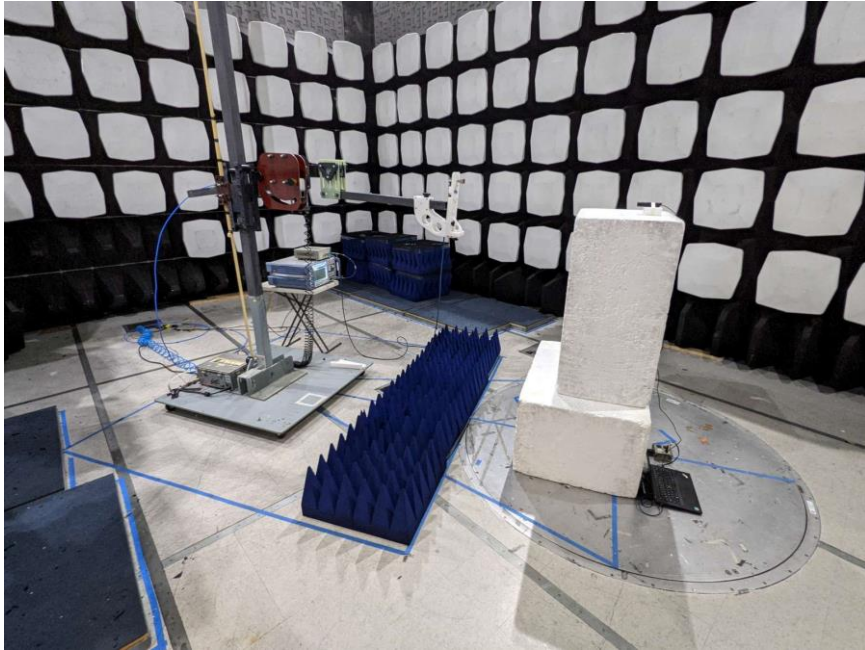
Figure A-5 – Test Set up - Radiated Emissions >18 GHz
