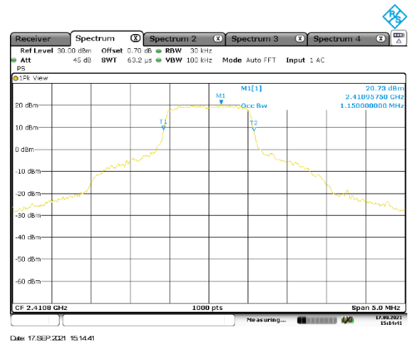
Figure 2.4.6-16: Mode 4 – 99% BW – LCH – MCS0
