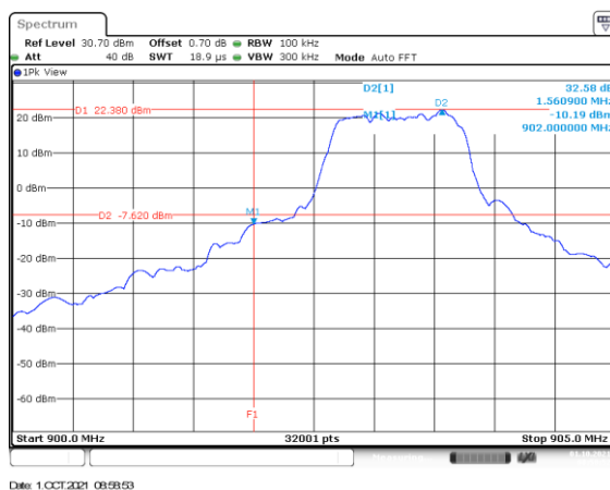
Figure 2.6.6-3: Lower Band edge – Mode 2 – MCS5
