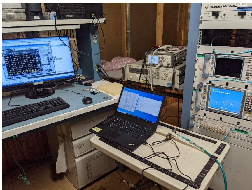
Figure 4 – Test Set up – Antenna Port measurement
