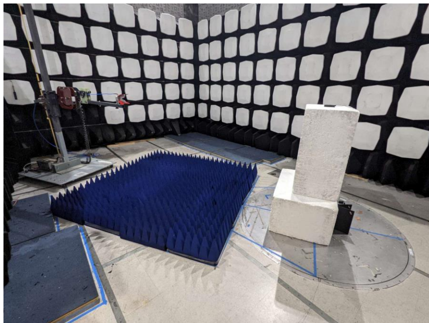
Figure 3 – Test Set up - Radiated Emissions <10 GHz
