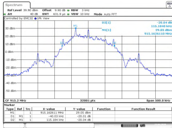
Figure 7.4.4.2-13: 20dB BW Mid Channel – 150kbps
