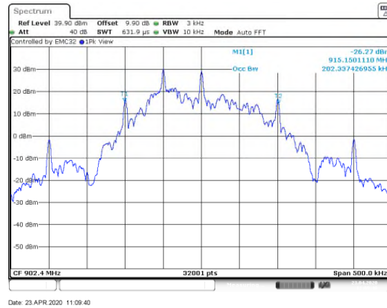
Figure 7.4.4.2-28: 99% BW Low Channel – 200kbps
