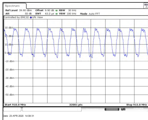
Figure 7.4.2.2-15: Mode 3 (64 Channels)
