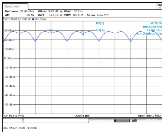
Figure 7.4.1.2-2: Channel Separation – Mode 2
