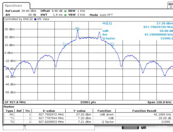
Figure 7.4.4.2-16: 20dB BW High Channel – 19.2kbps
