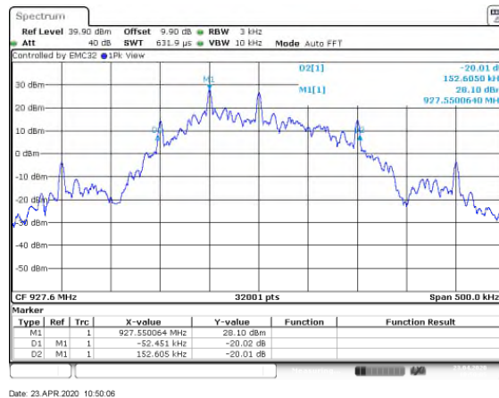
Figure 7.4.4.2-21: 20dB BW High Channel – 200kbps
