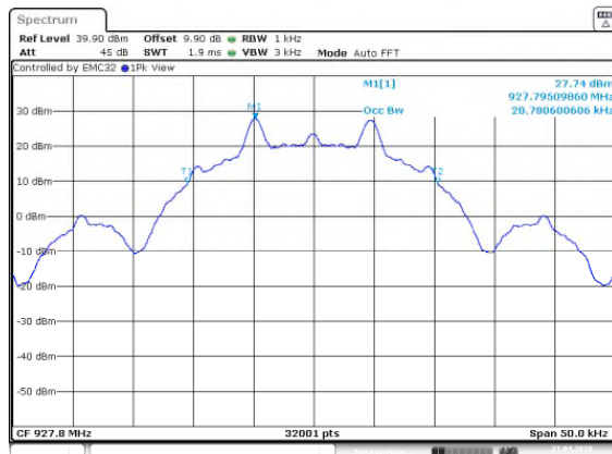
Figure 7.4.4.2-36: 99% BW High Channel - 9.6kbps
