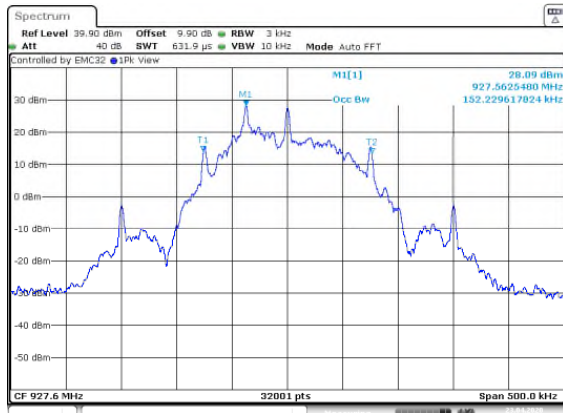
Figure 7.4.4.2-41: 99% BW High Channel – 150kbps
