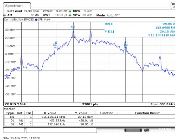
Figure 7.4.4.2-14: 20dB BW Mid Channel – 200kbps
