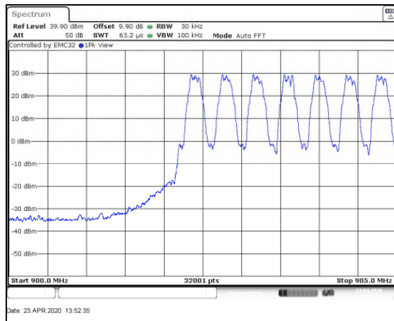
Figure 7.4.2.2-13: Mode 3 (64 Channels)
