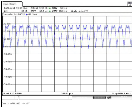
Figure 7.4.2.2-4: Mode 1 (86 Channels)
