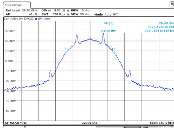
Figure 7.4.4.2-40: 99% BW High Channel – 115.2kbps
