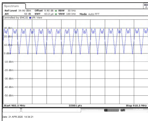
Figure 7.4.2.2-2: Mode 1 (86 Channels)
