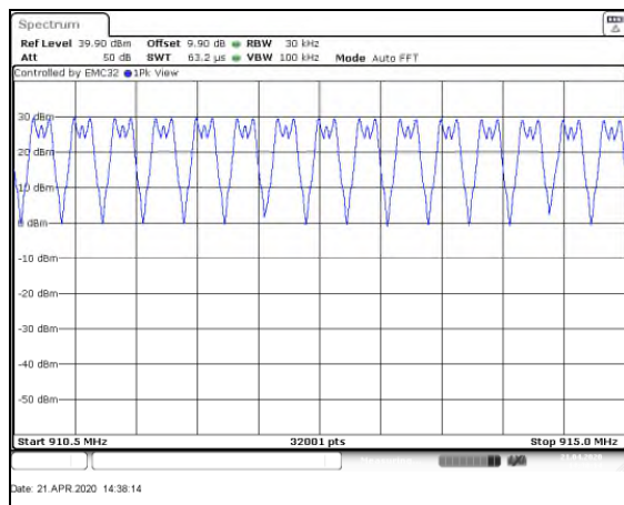
Figure 7.4.2.2-3: Mode 1 (86 Channels)
