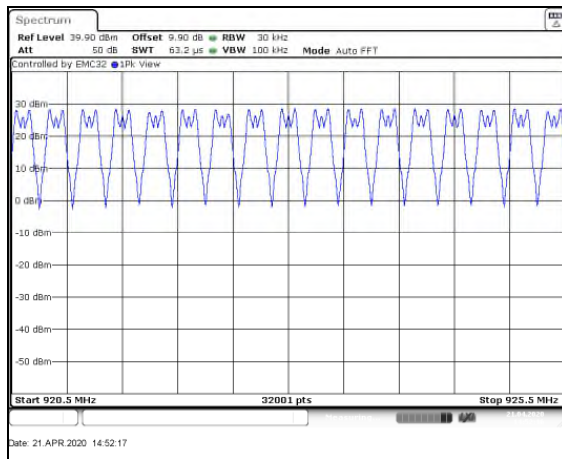
Figure 7.4.2.2-5: Mode 1 (86 Channels)
