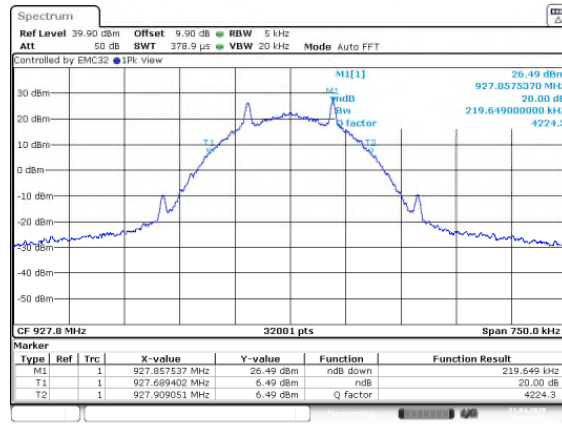
Figure 7.4.4.2-19: 20dB BW High Channel – 115.2kbps
