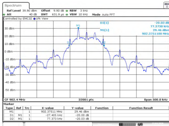
Figure 7.4.4.2-4: 20dB BW Low Channel - 50.0kbps
