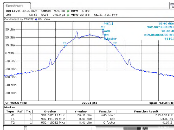
Figure 7.4.4.2-5: 20dB BW Low Channel - 115.2kbps
