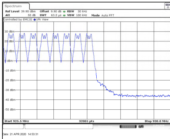
Figure 7.4.2.2-6: Mode 1 (86 Channels)
