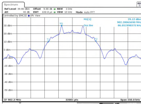
Figure 7.4.4.2-24: 99% BW Low Channel - 38.4kbps
