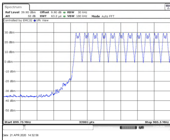
Figure 7.4.2.2-1: Mode 1 (86 Channels)
