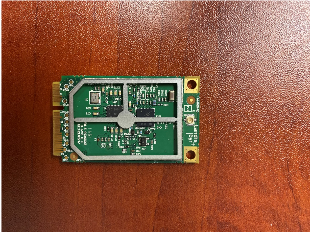
Figure 3: RF Board No Shields Front View
