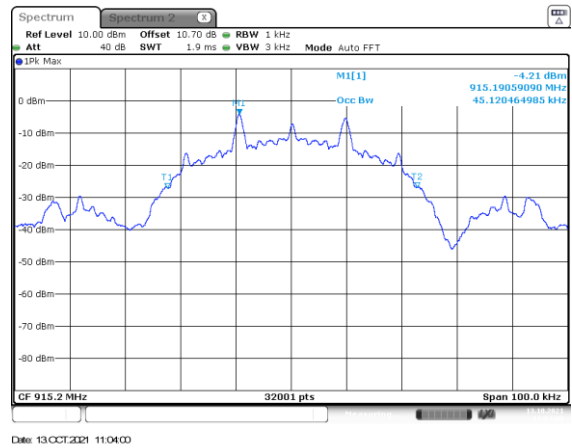
Figure 2.3.6-18: 99% BW Mid Channel – 19.2 kbps
