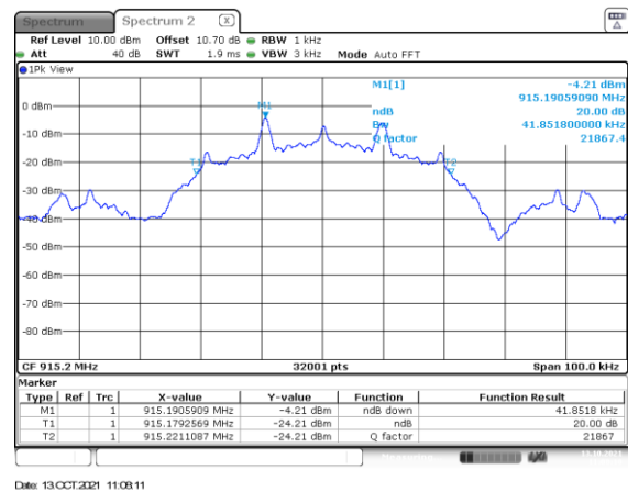
Figure 2.3.6-6: 20dB BW Mid Channel – 19.2 kbps
