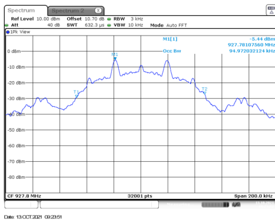
Figure 2.3.6-23: 99% BW High Channel – 38.4 kbps
