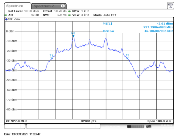
Figure 2.3.6-22: 99% BW High Channel – 19.2 kbps
