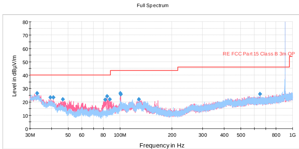
Figure A-3: Reference plot for Radiated Spurious Emissions – 30MHz - 1GHz
