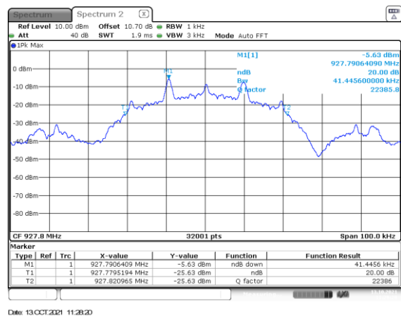
Figure 2.3.6-10: 20dB BW High Channel – 19.2 kbps
