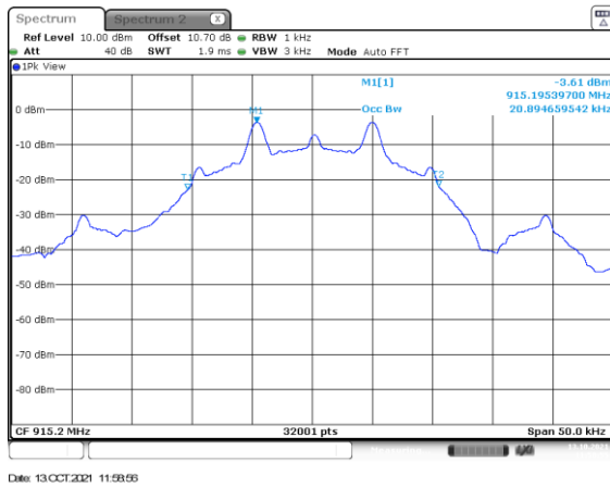
Figure 2.3.6-17: 99% BW Mid Channel – 9.6 kbps
