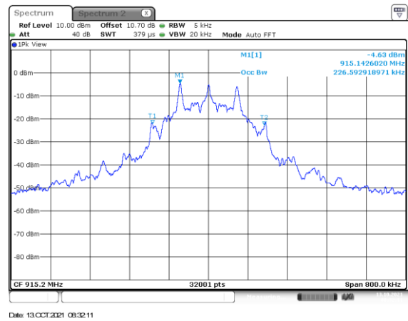
Figure 2.3.6-20: 99% BW Mid Channel – 115.2 kbps
