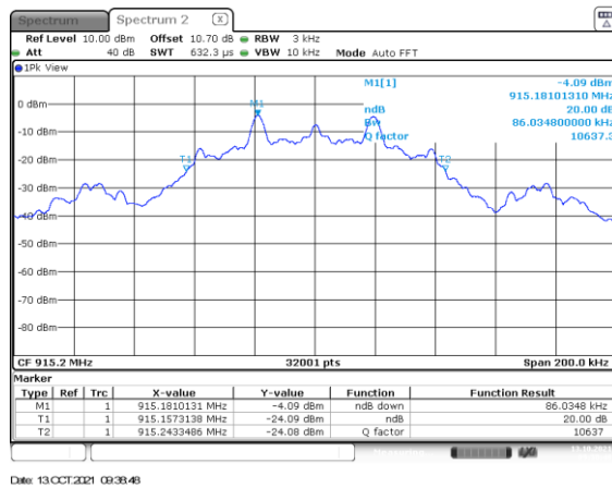
Figure 2.3.6-7: 20dB BW Mid Channel – 38.4 kbps
