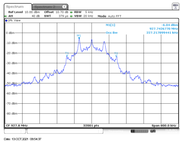
Figure 2.3.6-24: 99% BW High Channel – 115.2 kbps
