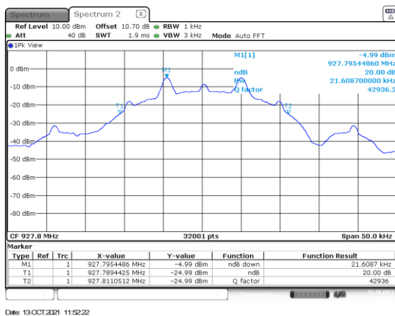
Figure 2.3.6-9: 20dB BW High Channel – 9.6 kbps
