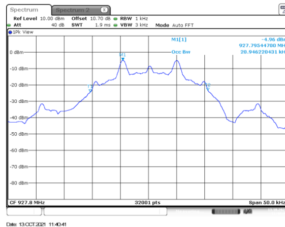
Figure 2.3.6-21: 99% BW High Channel – 9.6 kbps
