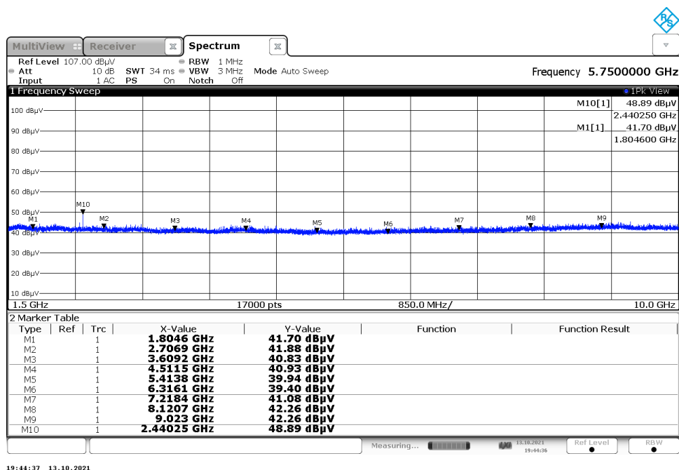
Figure A-5: Reference plot for Radiated Spurious Emissions – 1.5 GHz – 10 GHz
