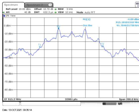
Figure 2.3.6-19: 99% BW Mid Channel – 38.4 kbps
