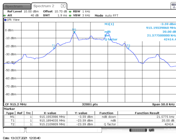
Figure 2.3.6-5: 20dB BW Mid Channel – 9.6 kbps
