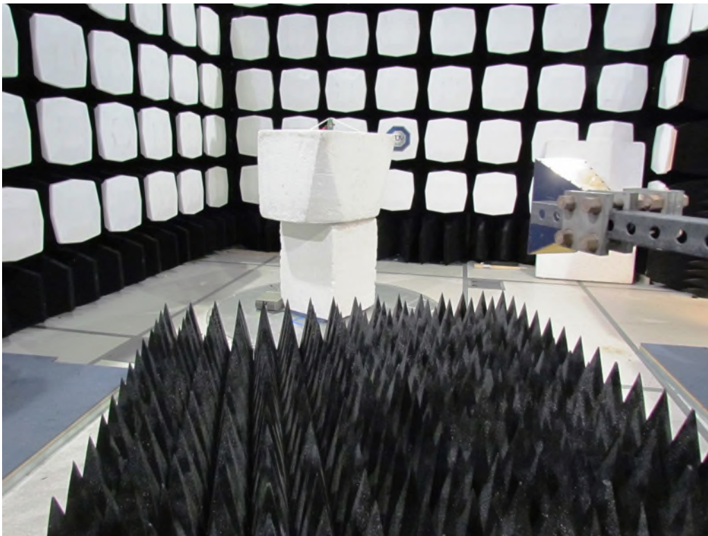
Figure 6: Equipment Under Test – Radiated Emissions >1GHz
