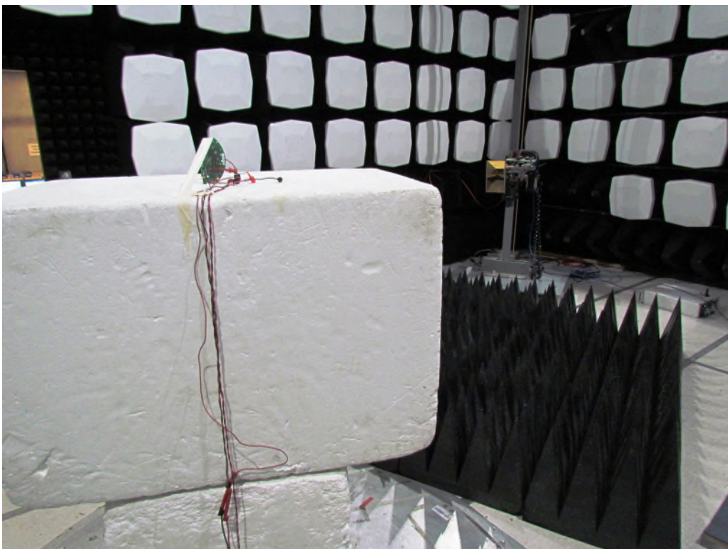
Figure 7: Equipment Under Test – Radiated Emissions >1GHz
