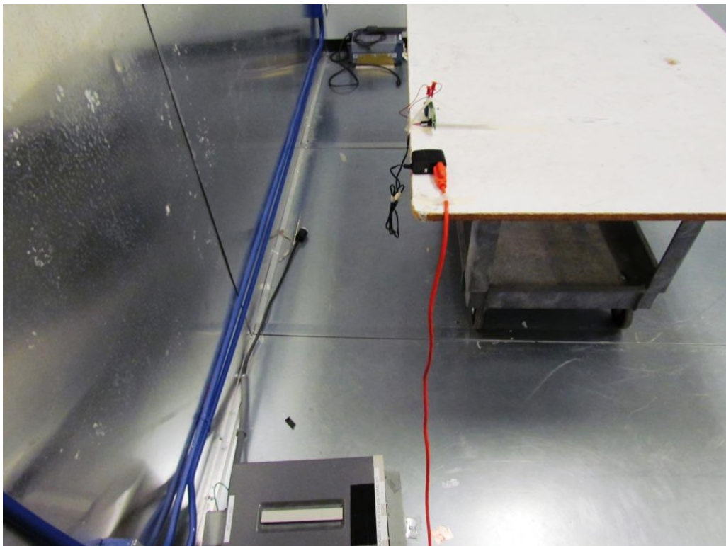
Figure 9: Equipment Under Test – AC Conducted Emissions
