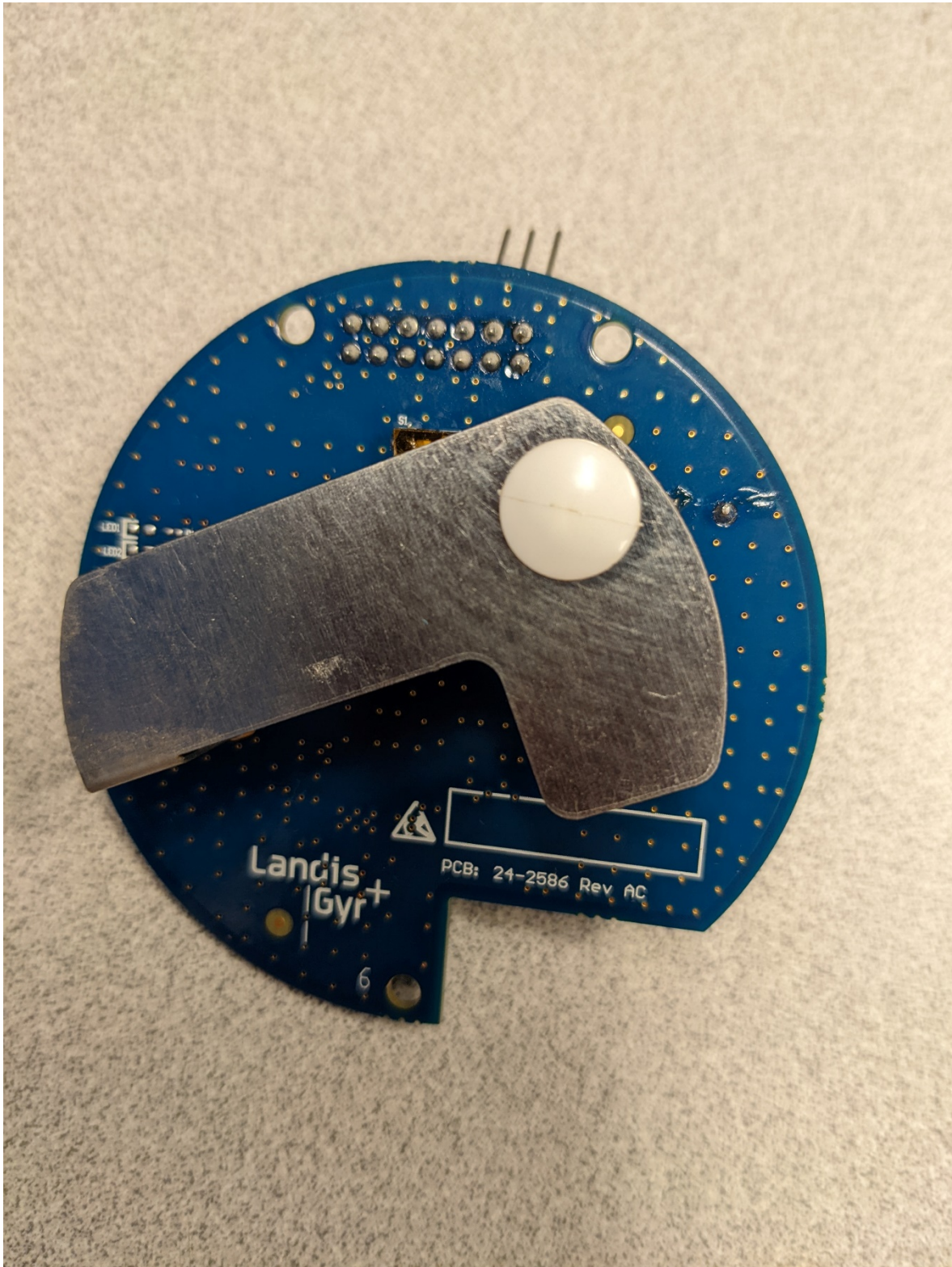
Figure 4: New Stamped Metal Planar Inverted F Antenna
