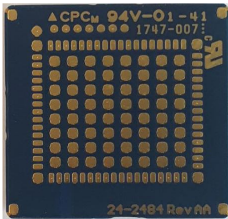
Figure 2: Bottom View
