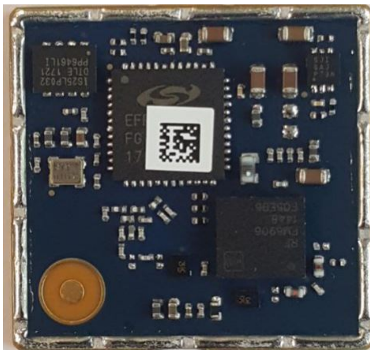
Figure 1: Top View
