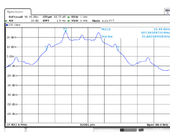
Figure 7.4.4.2-56: 99% BW High Channel - 10kbps
