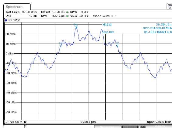
Figure 7.4.4.2-52: 99% BW High Channel - 9.6kbps
