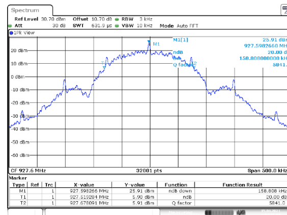
Figure 7.4.4.2-26: 20 dB BW High Channel – 20kbps
