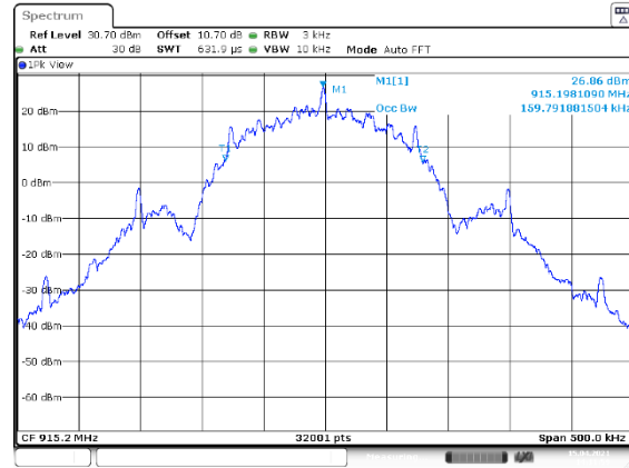
Figure 7.4.4.2-50: 99% BW Mid Channel – 150kbps
