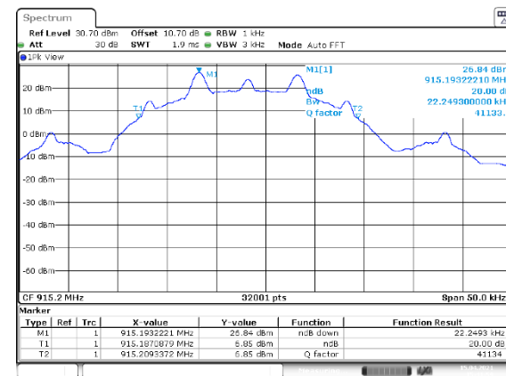
Figure 7.4.4.2-16: 20 dB BW Mid Channel – 10kbps
