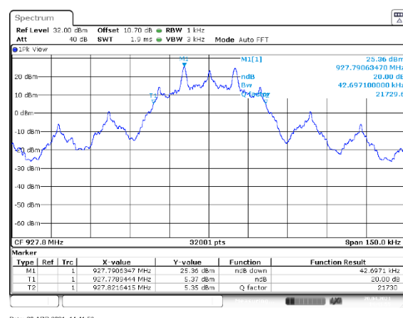
Figure 7.4.4.2-22: 20 dB BW High Channel – 19.2kbps
