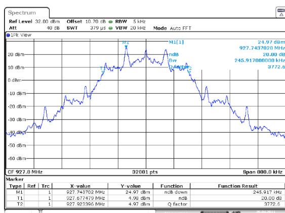
Figure 7.4.4.2-24: 20 dB BW High Channel – 115.2kbps
