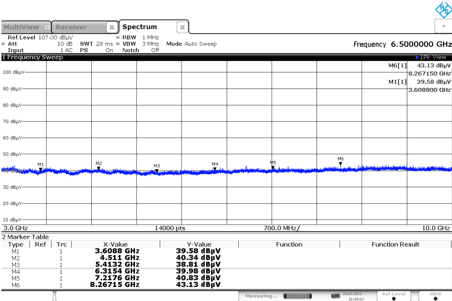
Figure A-8: Radiated Emissions – 3 GHz – 10 GHz (WiSUN)
