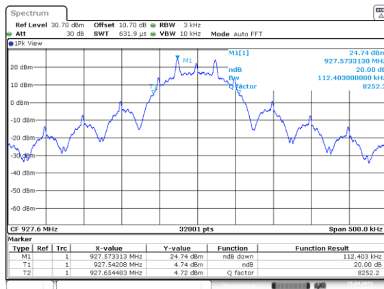
Figure 7.4.4.2-25: 20dB BW High Channel –10kbps
