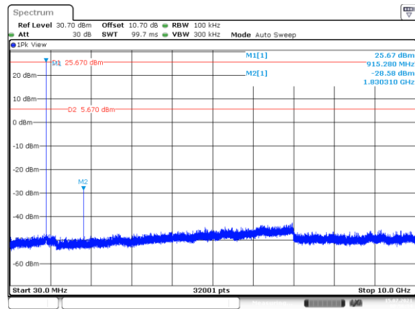
Figure 7.5.1.2-2: 30 MHz – 10 GHz – Mid Channel
