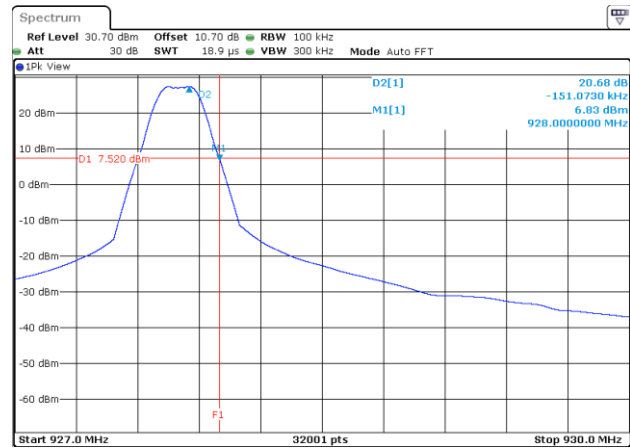
Figure 7.5.1.2-8: Upper Band edge – Mode 4
