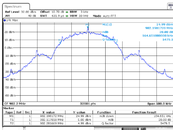
Figure 7.4.4.2-11: 20 dB BW Low Channel – 150kbps
