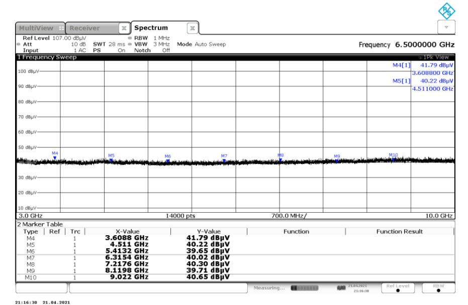
Figure A-7: Radiated Emissions – 3 GHz – 10 GHz (Mesh)
