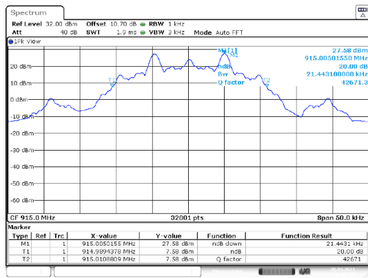
Figure 7.4.4.2-12: 20 dB BW Mid Channel – 9.6kbps
