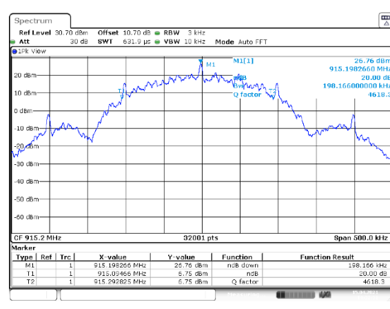
Figure 7.4.4.2-20: 20 dB BW Mid Channel – 200kbps
