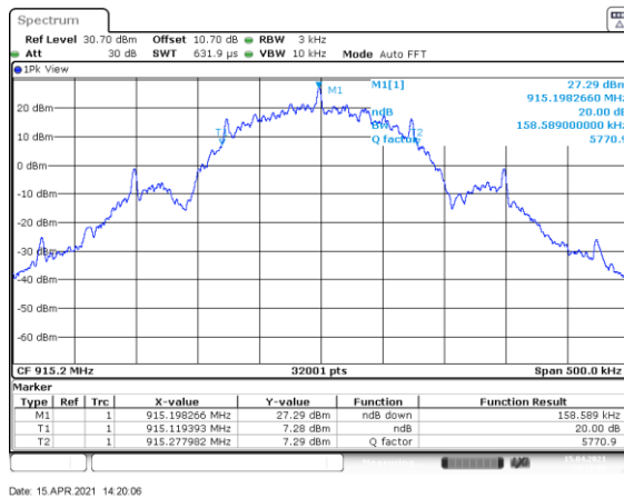
Figure 7.4.4.2-19: 20 dB BW Mid Channel –150kbps
