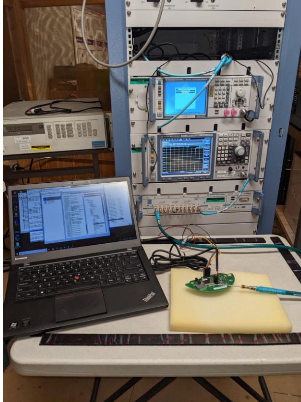
Figure 1: Equipment Under Test – Antenna Port Conducted Measurements
