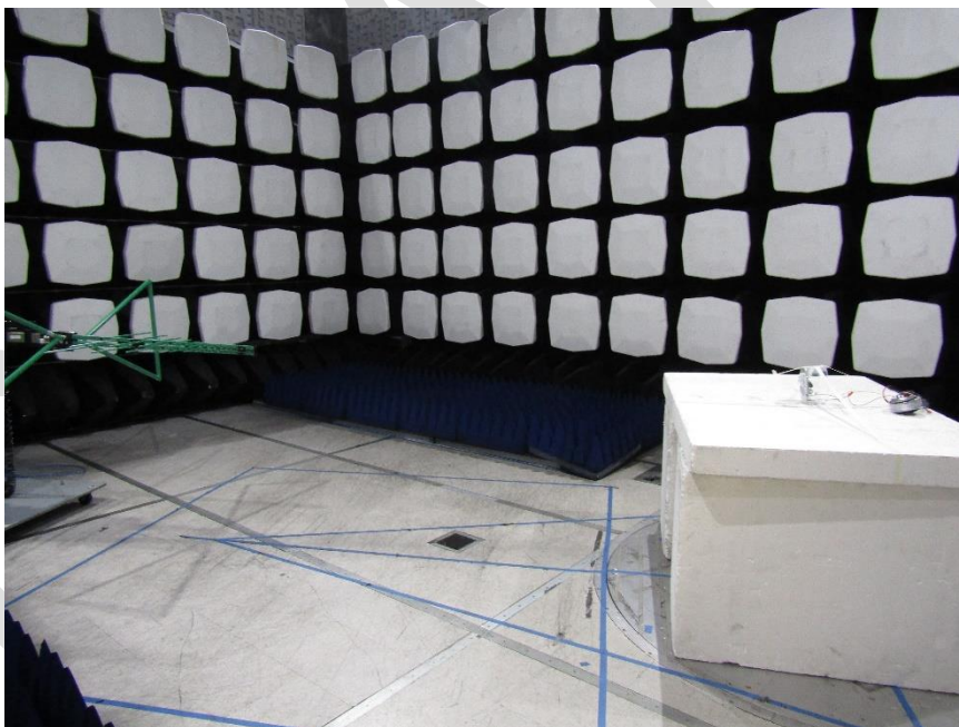
Figure:2 – Test Set up - Radiated Emissions <1 GHz
