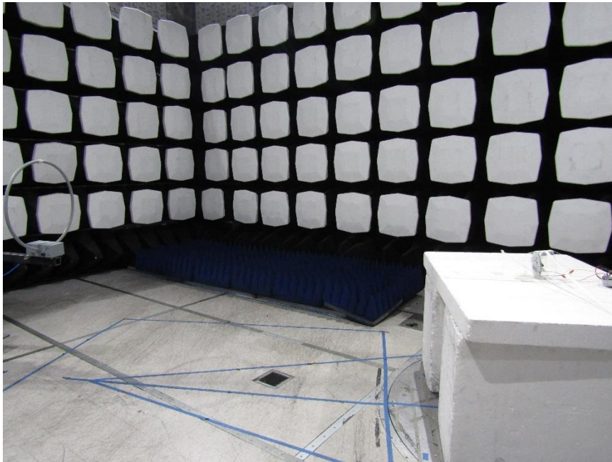
Figure:1 – Test Set up - Radiated Emissions <30 MHz
