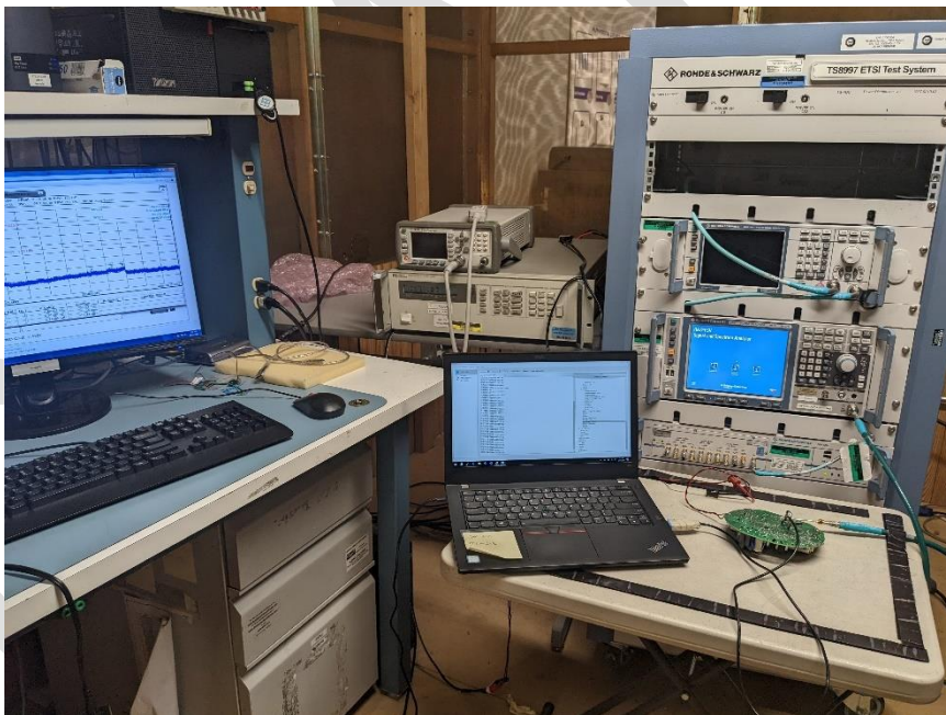
Figure:4 – Test Set up – Antenna Port measurements
