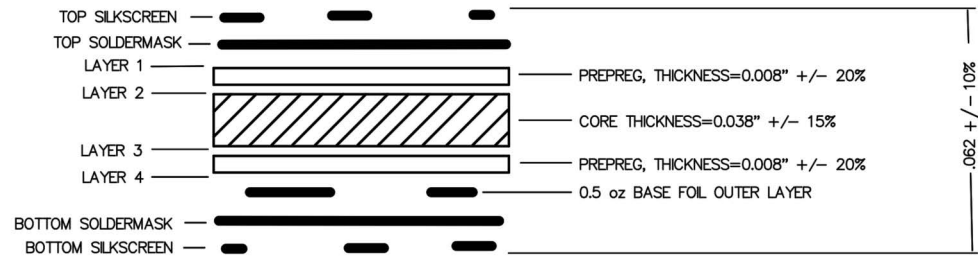
Figure 5. PCB Stack Up
