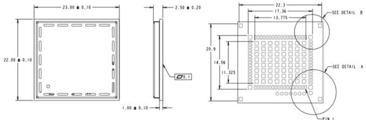
Figure 2. PCB Outline 1
