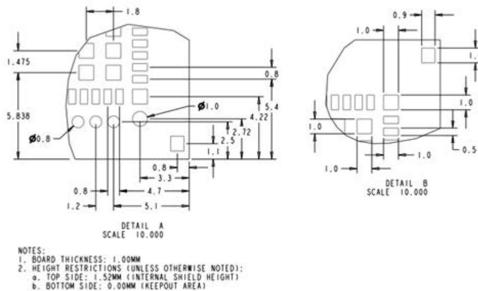
Figure 3. PCB Outline 2
