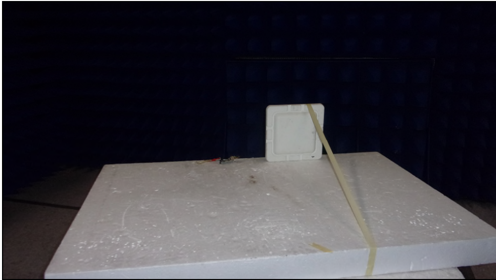
Figure 1: Equipment Under Test – Radiated Emissions <30MHz
