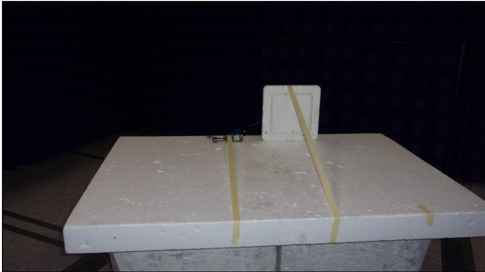
Figure 3: Equipment Under Test – Radiated Emissions <1GHz
