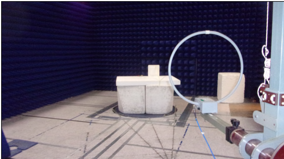
Figure 2: Equipment Under Test – Radiated Emissions <30MHz
