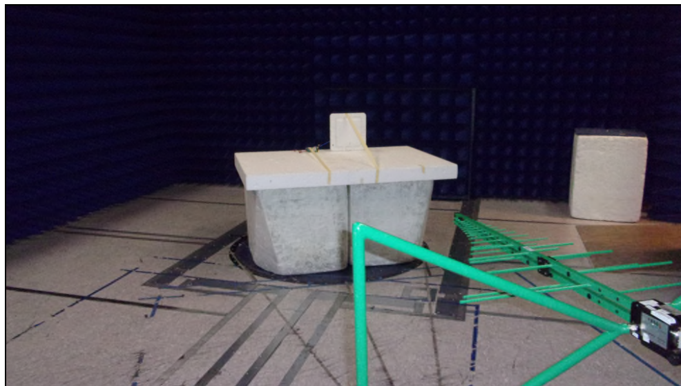
Figure 4: Equipment Under Test – Radiated Emissions <1GHz
