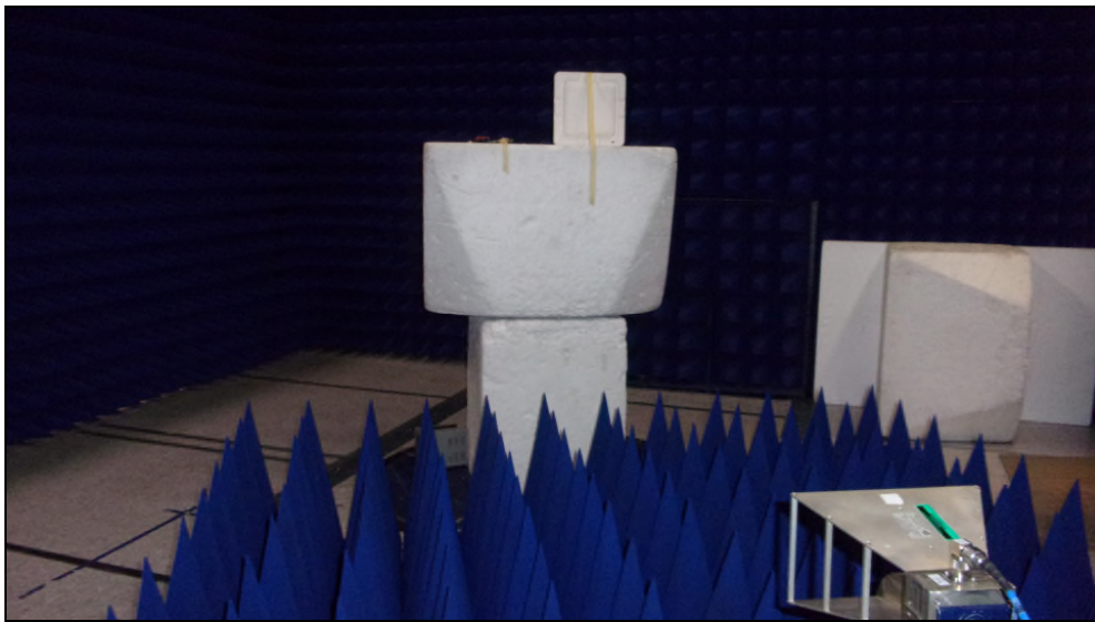
Figure 6: Equipment Under Test – Radiated Emissions >1GHz
