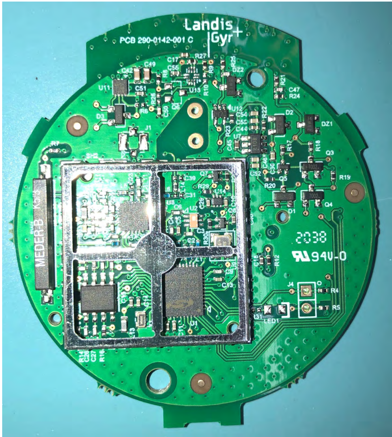
Figure 2: Top View without Shield
