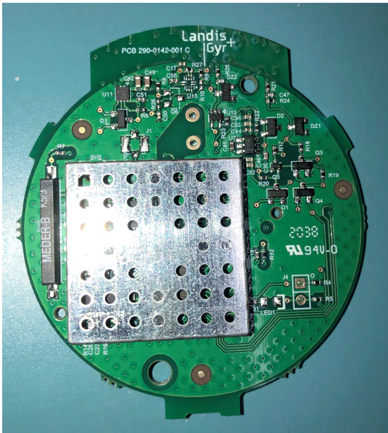
Figure 1: Top View with Shield
