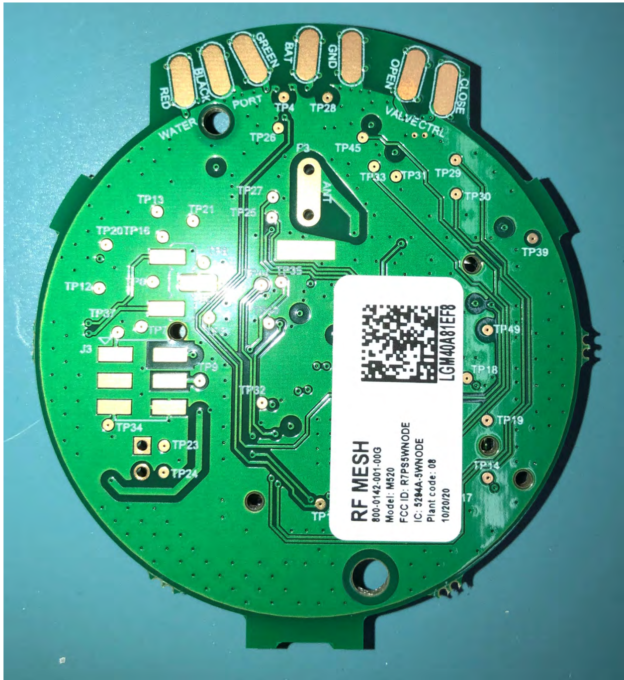
Figure 3: Bottom View
