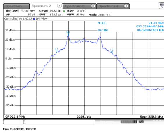
Figure 7.4.4.2-24: 99% BW High Channel – 50.0kbps
