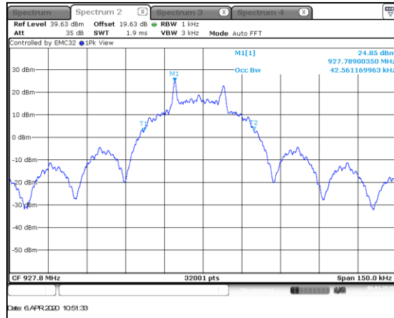
Figure 7.4.4.2-22: 99% BW High Channel – 19.2kbps
