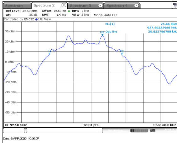
Figure 7.4.4.2-21: 99% BW High Channel - 9.6kbps
