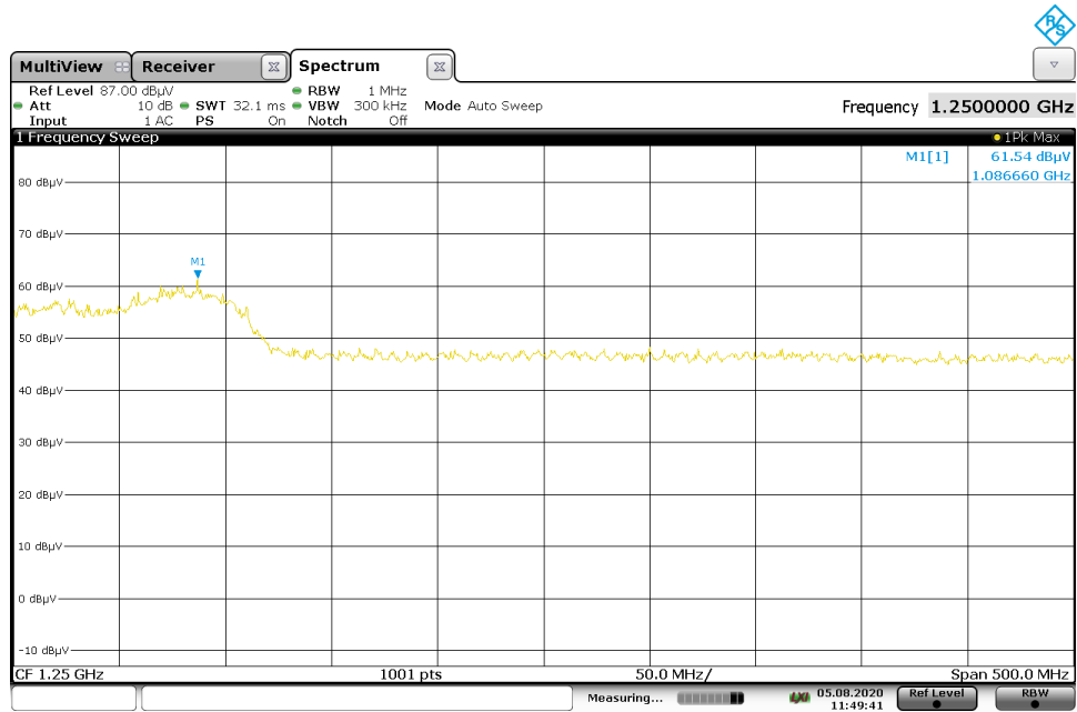
Figure A-7: Radiated Emissions – 1 GHz – 1.5 GHz Metal Antenna Sleeve
