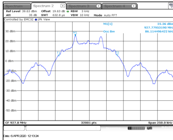
Figure 7.4.4.2-23: 99% BW High Channel – 38.4kbps
