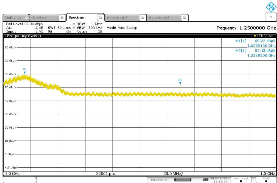
Figure A-8: Radiated Emissions – 1 GHz – 1.5 GHz Plastic Antenna Sleeve
